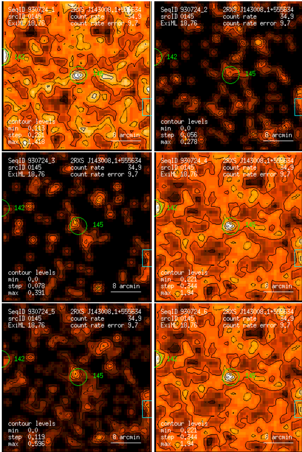
Figure 145: RASS 930724: detection 0145: band rate images, Gaussian filter: (1) PSPC channels 11 – 41, (2) 52 – 90, (3) 91 – 201, (4) 11 – 235, (5) 52 – 201, (6) 11 – 201. Broad band rates in counts/ks. Band rate contour levels in counts/ks/arcmin 2 .
