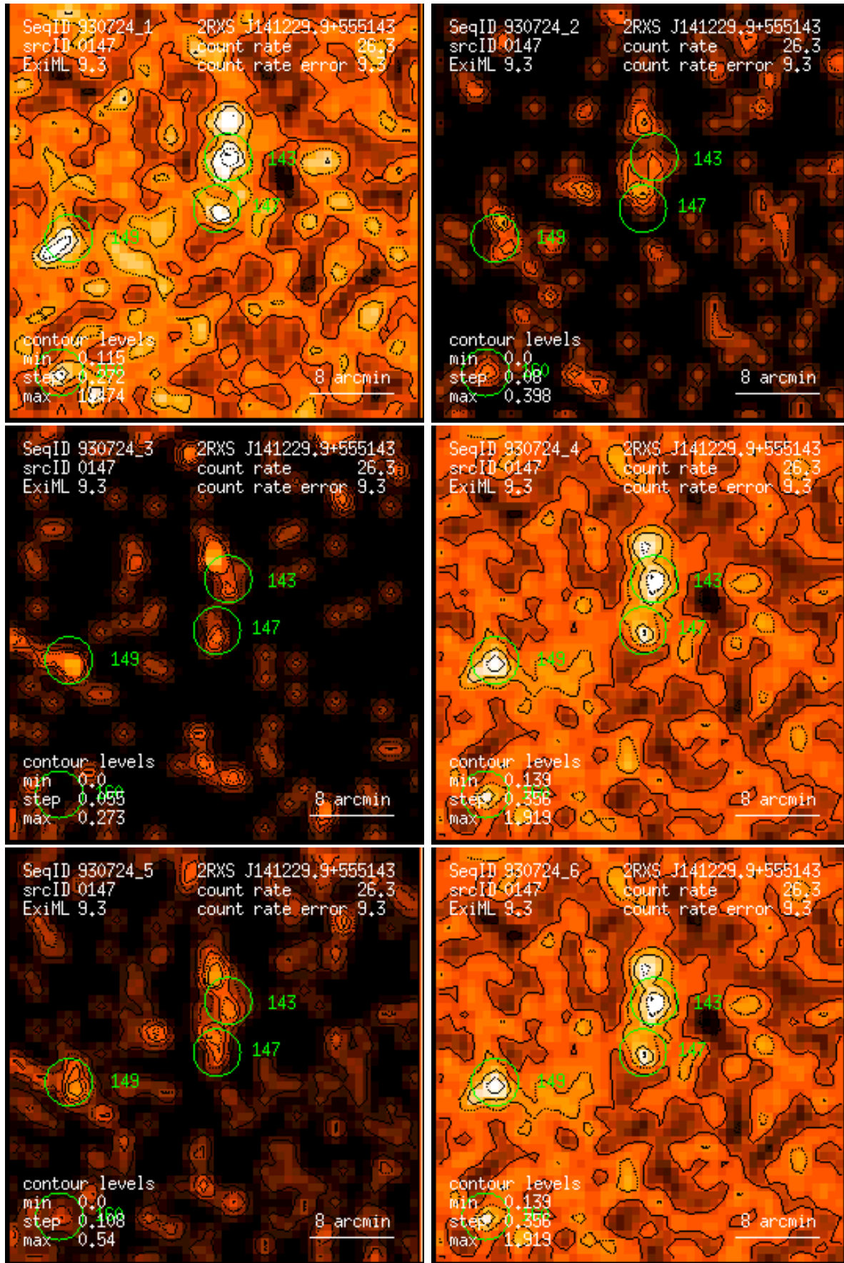
Figure 147: RASS 930724: detection 0147: band rate images, Gaussian filter: (1) PSPC channels 11 – 41, (2) 52 – 90, (3) 91 – 201, (4) 11 – 235, (5) 52 – 201, (6) 11 – 201. Broad band rates in counts/ks. Band rate contour levels in counts/ks/arcmin 2 .
