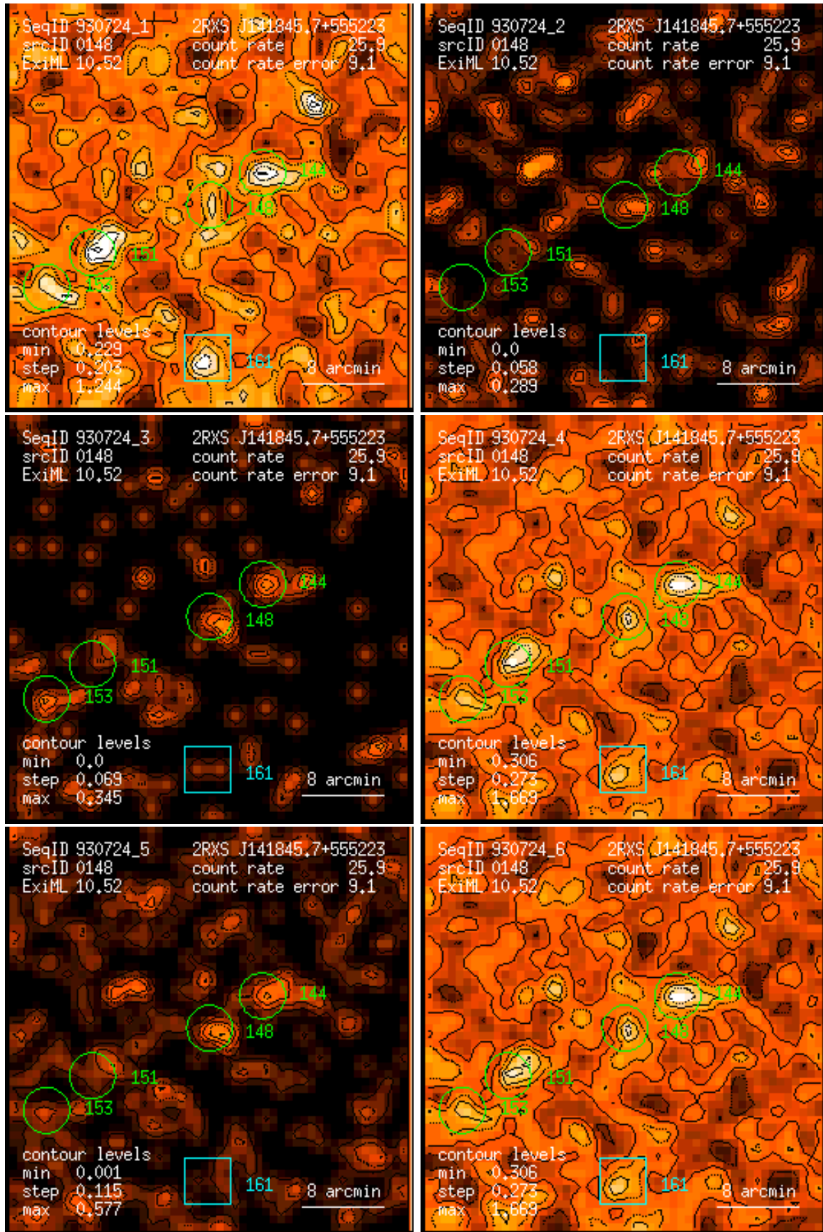
Figure 148: RASS 930724: detection 0148: band rate images, Gaussian filter: (1) PSPC channels 11 – 41, (2) 52 – 90, (3) 91 – 201, (4) 11 – 235, (5) 52 – 201, (6) 11 – 201. Broad band rates in counts/ks. Band rate contour levels in counts/ks/arcmin 2 .
