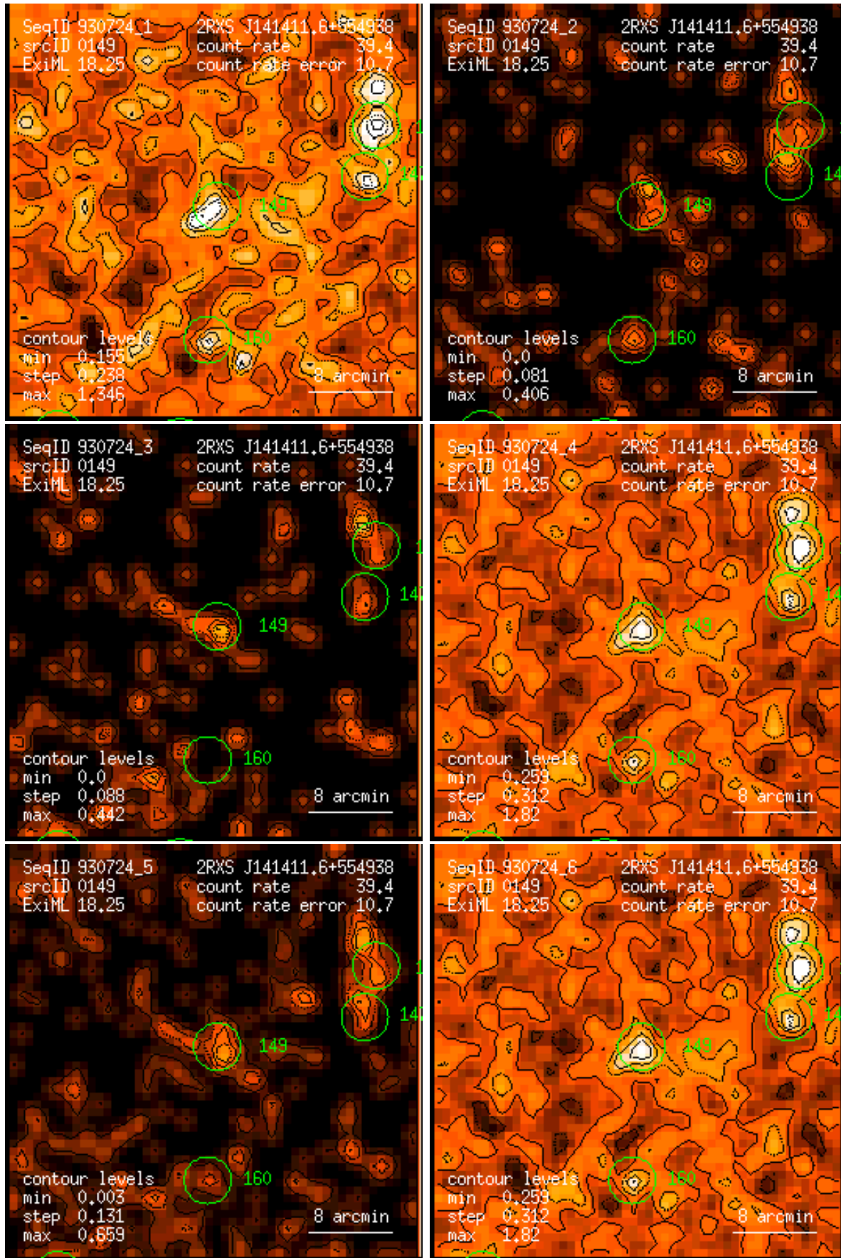
Figure 149: RASS 930724: detection 0149: band rate images, Gaussian filter: (1) PSPC channels 11 – 41, (2) 52 – 90, (3) 91 – 201, (4) 11 – 235, (5) 52 – 201, (6) 11 – 201. Broad band rates in counts/ks. Band rate contour levels in counts/ks/arcmin 2 .
