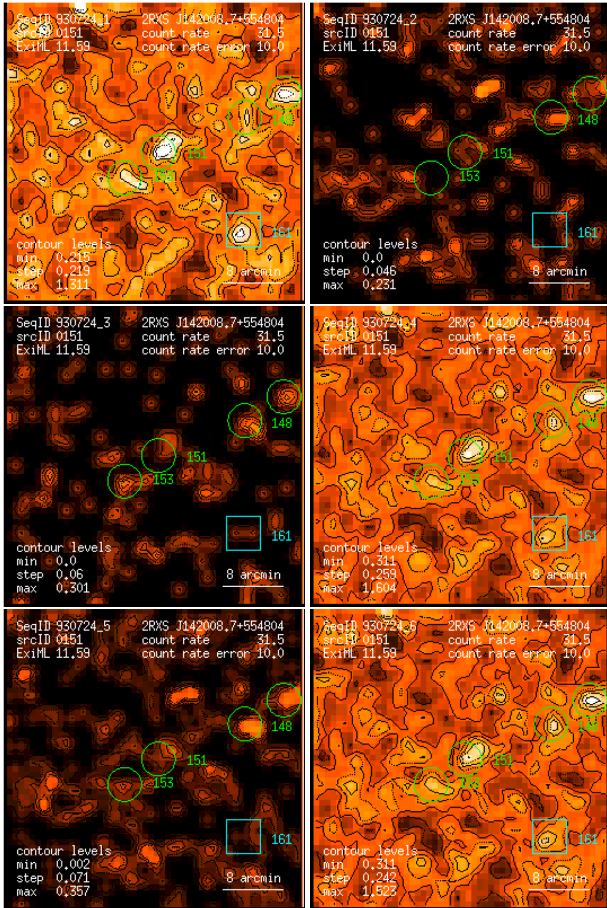
Figure 151: RASS 930724: detection 0151: band rate images, Gaussian filter: (1) PSPC channels 11 – 41, (2) 52 – 90, (3) 91 – 201, (4) 11 – 235, (5) 52 – 201, (6) 11 – 201. Broad band rates in counts/ks. Band rate contour levels in counts/ks/arcmin 2 .
