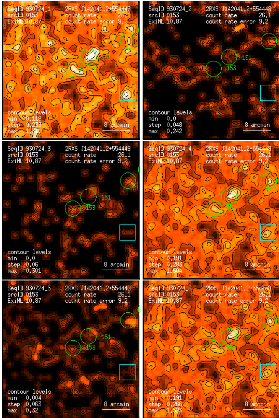
Figure 153: RASS 930724: detection 0153: band rate images, Gaussian filter: (1) PSPC channels 11 – 41, (2) 52 – 90, (3) 91 – 201, (4) 11 – 235, (5) 52 – 201, (6) 11 – 201. Broad band rates in counts/ks. Band rate contour levels in counts/ks/arcmin 2 .
