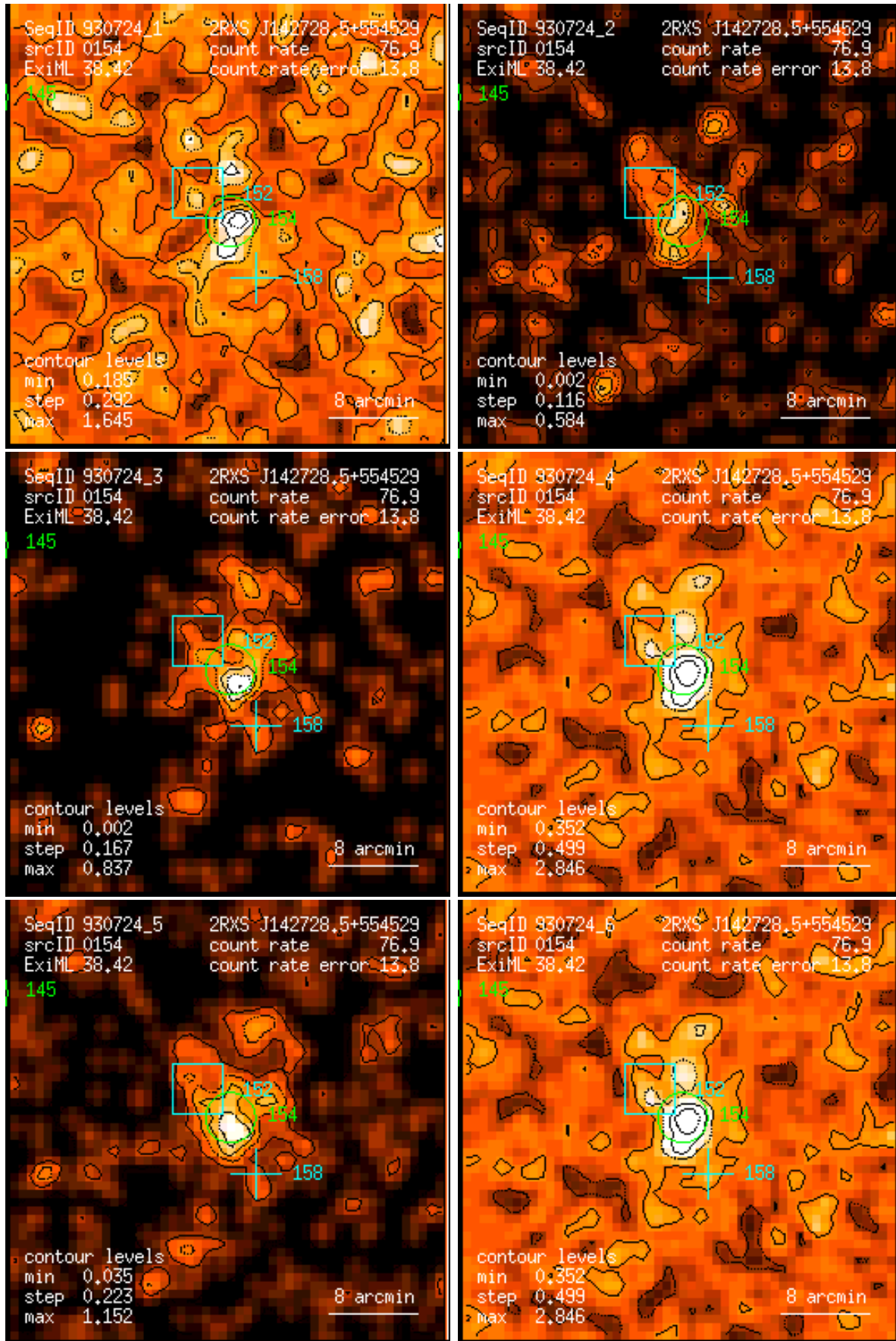
Figure 154: RASS 930724: detection 0154: band rate images, Gaussian filter: (1) PSPC channels 11 – 41, (2) 52 – 90, (3) 91 – 201, (4) 11 – 235, (5) 52 – 201, (6) 11 – 201. Broad band rates in counts/ks. Band rate contour levels in counts/ks/arcmin 2 .
