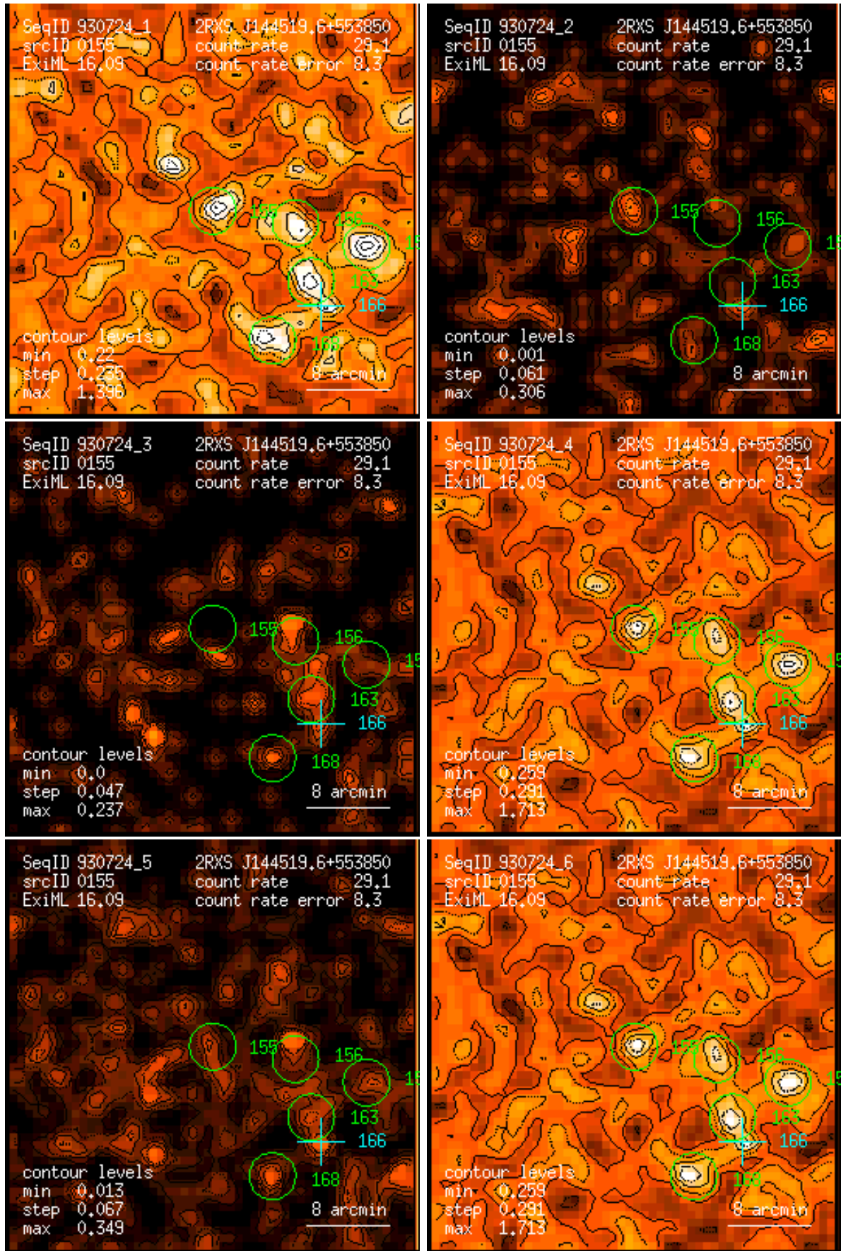
Figure 155: RASS 930724: detection 0155: band rate images, Gaussian filter: (1) PSPC channels 11 – 41, (2) 52 – 90, (3) 91 – 201, (4) 11 – 235, (5) 52 – 201, (6) 11 – 201. Broad band rates in counts/ks. Band rate contour levels in counts/ks/arcmin 2 .
