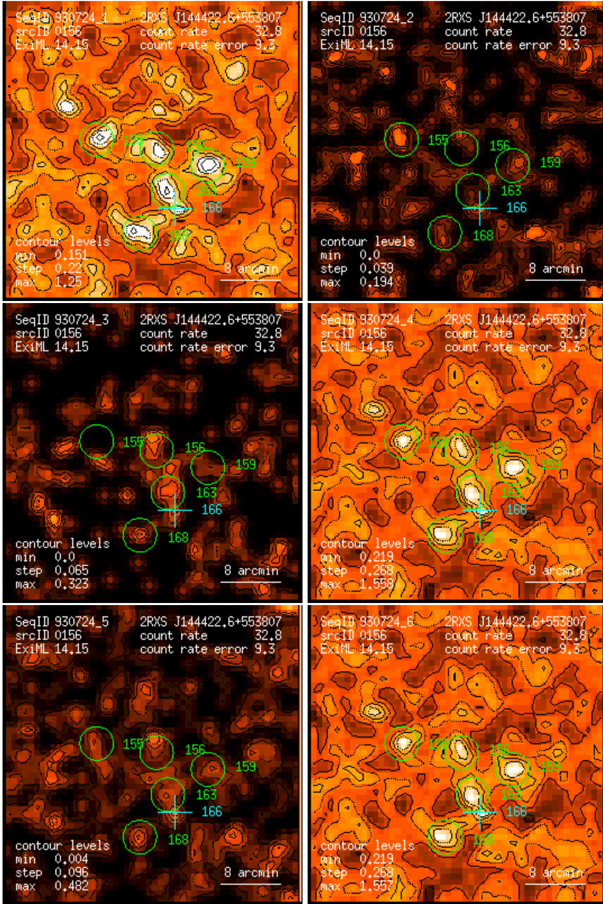
Figure 156: RASS 930724: detection 0156: band rate images, Gaussian filter: (1) PSPC channels 11 – 41, (2) 52 – 90, (3) 91 – 201, (4) 11 – 235, (5) 52 – 201, (6) 11 – 201. Broad band rates in counts/ks. Band rate contour levels in counts/ks/arcmin 2 .
