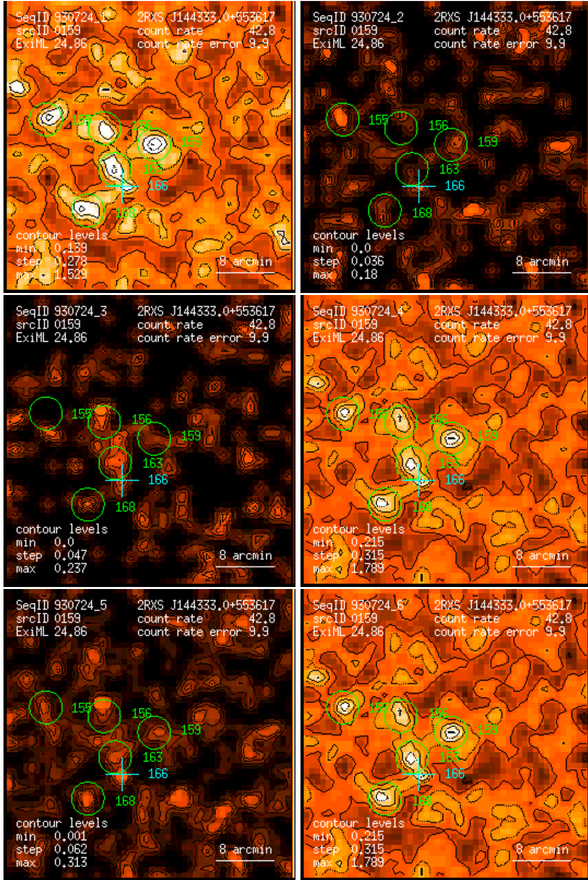
Figure 159: RASS 930724: detection 0159: band rate images, Gaussian filter: (1) PSPC channels 11 – 41, (2) 52 – 90, (3) 91 – 201, (4) 11 – 235, (5) 52 – 201, (6) 11 – 201. Broad band rates in counts/ks. Band rate contour levels in counts/ks/arcmin 2 .
