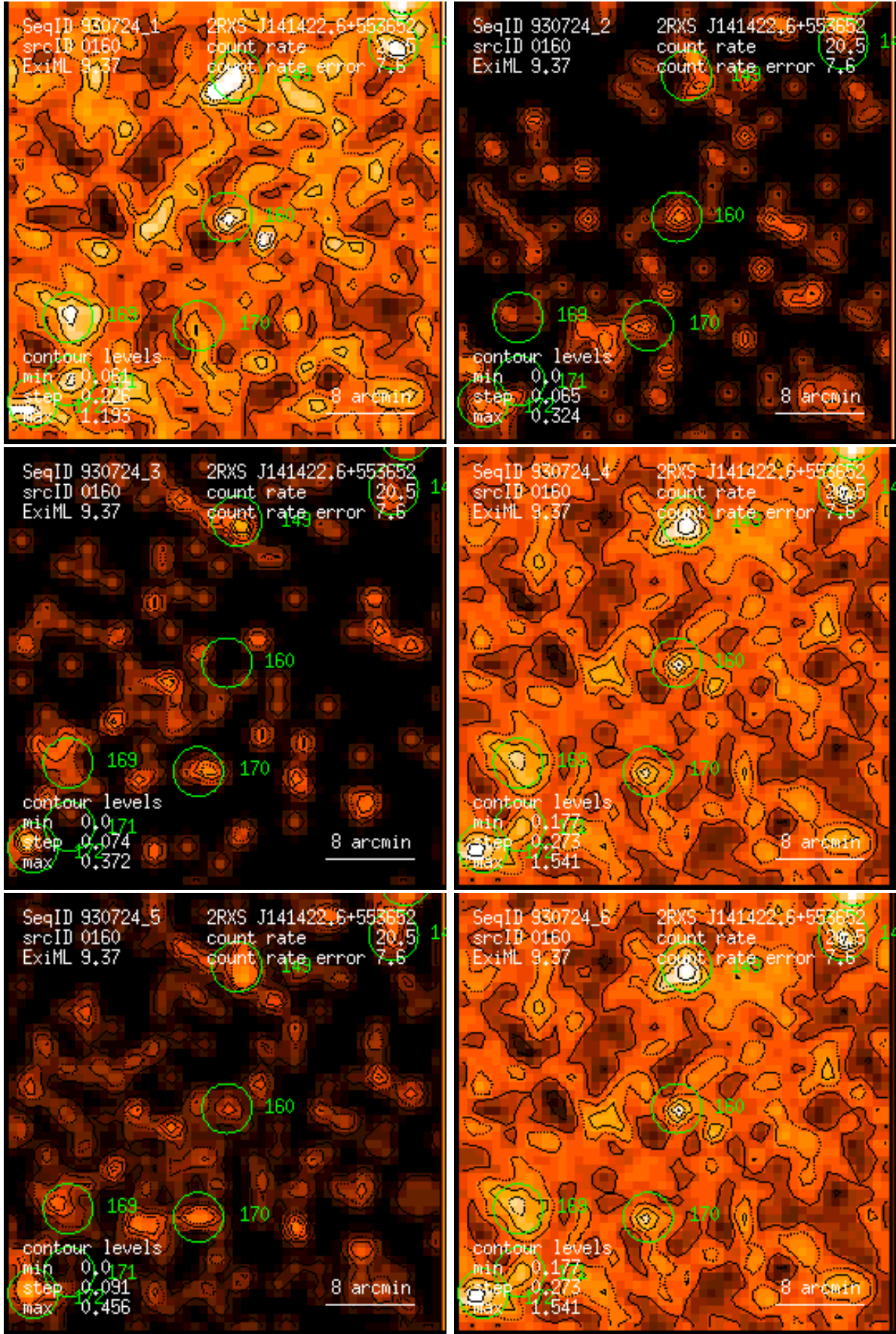
Figure 160: RASS 930724: detection 0160: band rate images, Gaussian filter: (1) PSPC channels 11 – 41, (2) 52 – 90, (3) 91 – 201, (4) 11 – 235, (5) 52 – 201, (6) 11 – 201. Broad band rates in counts/ks. Band rate contour levels in counts/ks/arcmin 2 .
