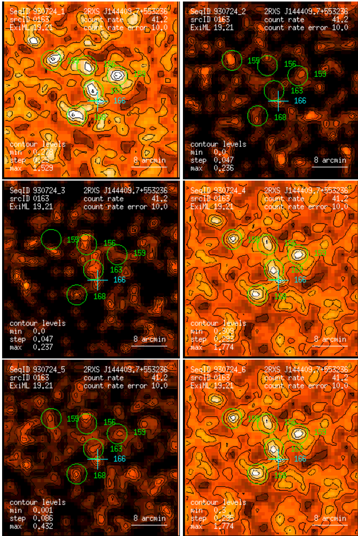
Figure 163: RASS 930724: detection 0163: band rate images, Gaussian filter: (1) PSPC channels 11 – 41, (2) 52 – 90, (3) 91 – 201, (4) 11 – 235, (5) 52 – 201, (6) 11 – 201. Broad band rates in counts/ks. Band rate contour levels in counts/ks/arcmin 2 .
