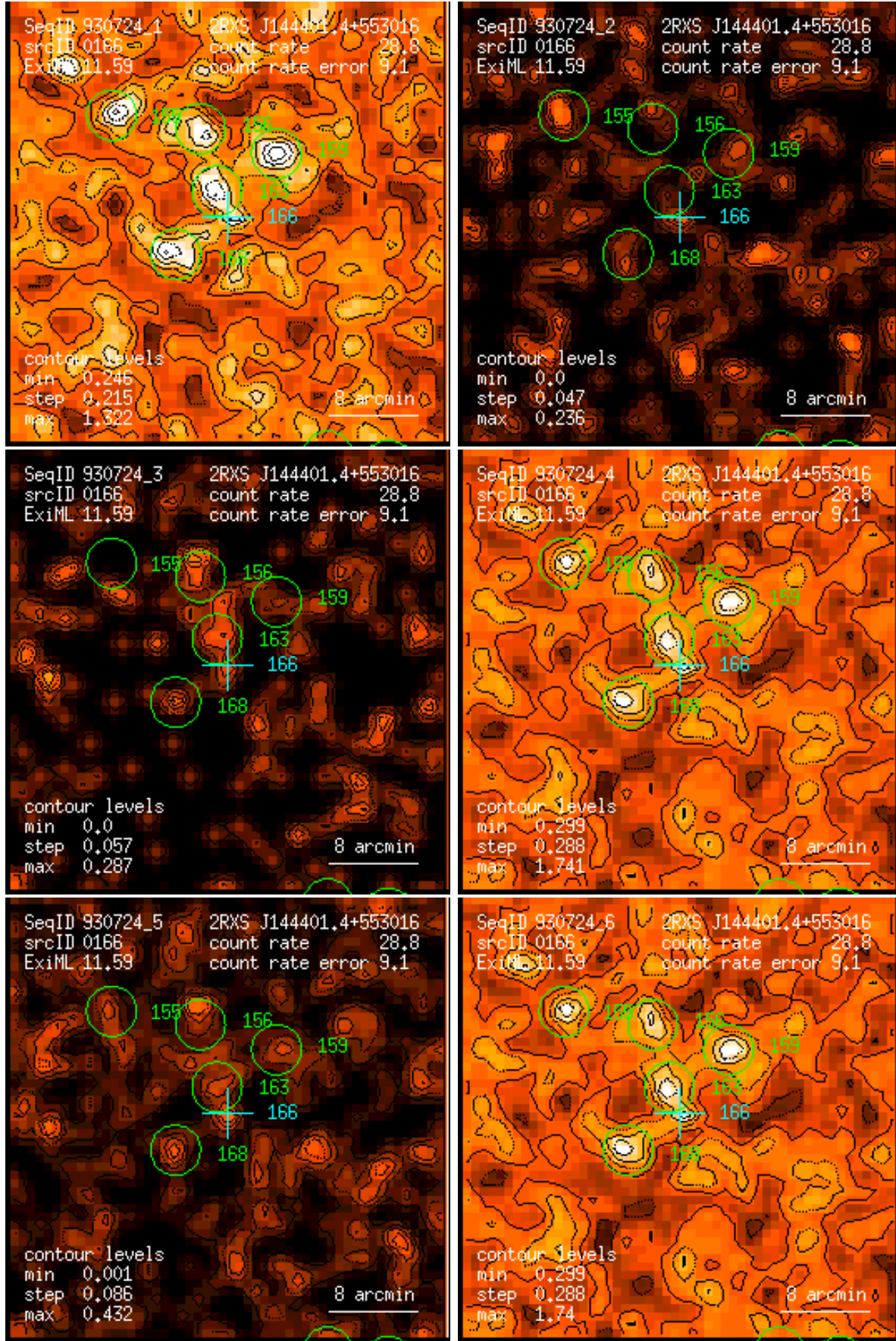
Figure 166: RASS 930724: detection 0166: band rate images, Gaussian filter: (1) PSPC channels 11 – 41, (2) 52 – 90, (3) 91 – 201, (4) 11 – 235, (5) 52 – 201, (6) 11 – 201. Broad band rates in counts/ks. Band rate contour levels in counts/ks/arcmin 2 .
