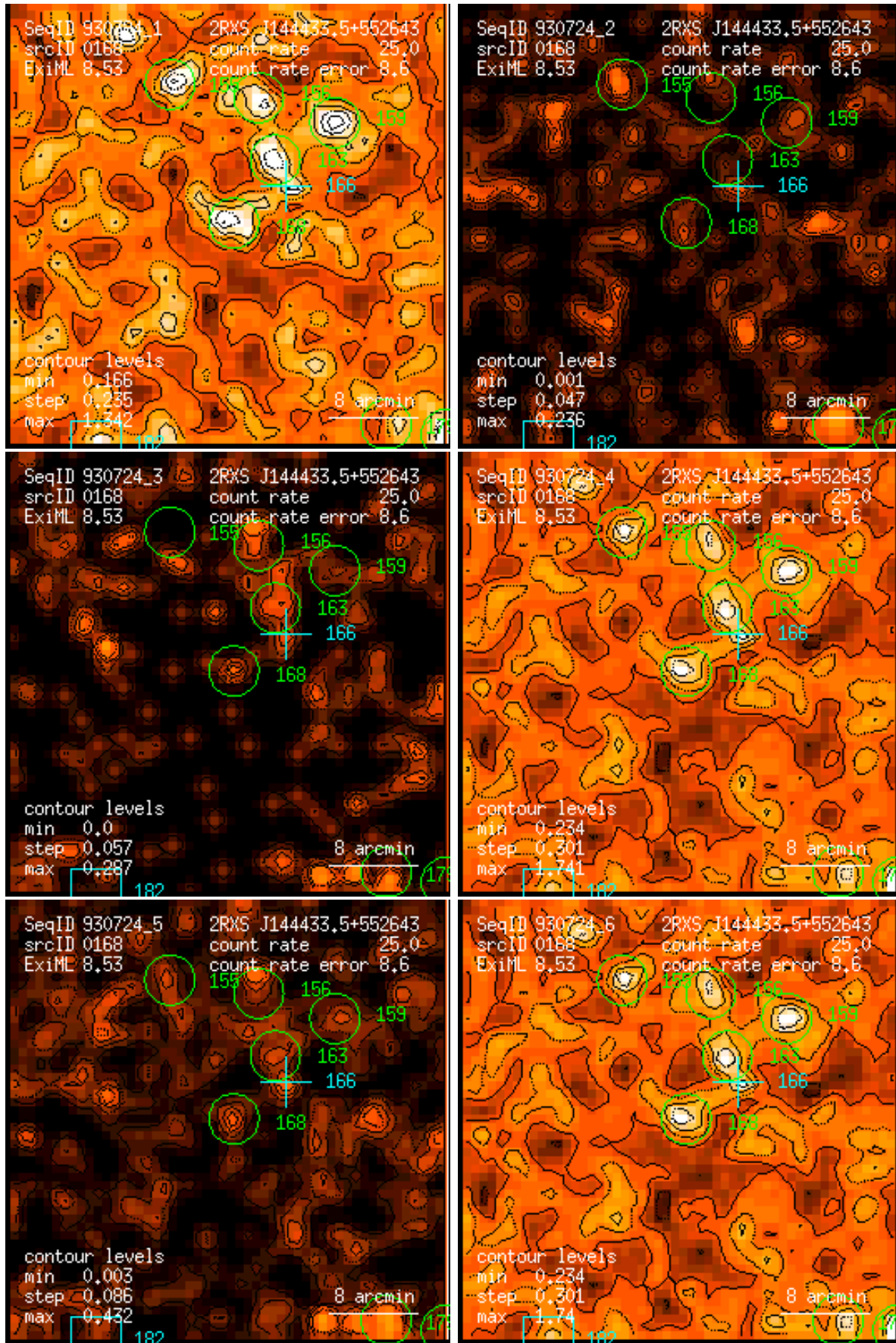
Figure 168: RASS 930724: detection 0168: band rate images, Gaussian filter: (1) PSPC channels 11 – 41, (2) 52 – 90, (3) 91 – 201, (4) 11 – 235, (5) 52 – 201, (6) 11 – 201. Broad band rates in counts/ks. Band rate contour levels in counts/ks/arcmin 2 .
