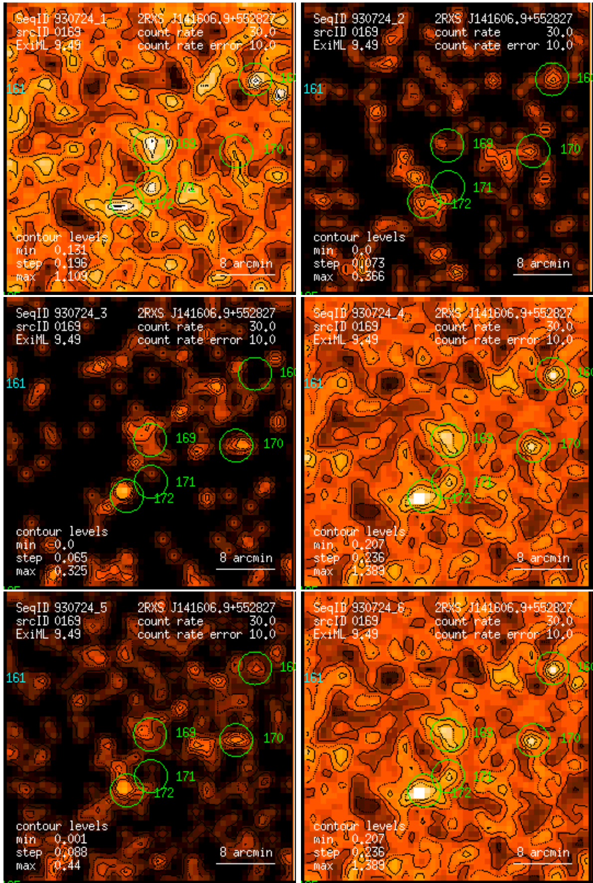
Figure 169: RASS 930724: detection 0169: band rate images, Gaussian filter: (1) PSPC channels 11 – 41, (2) 52 – 90, (3) 91 – 201, (4) 11 – 235, (5) 52 – 201, (6) 11 – 201. Broad band rates in counts/ks. Band rate contour levels in counts/ks/arcmin 2 .
