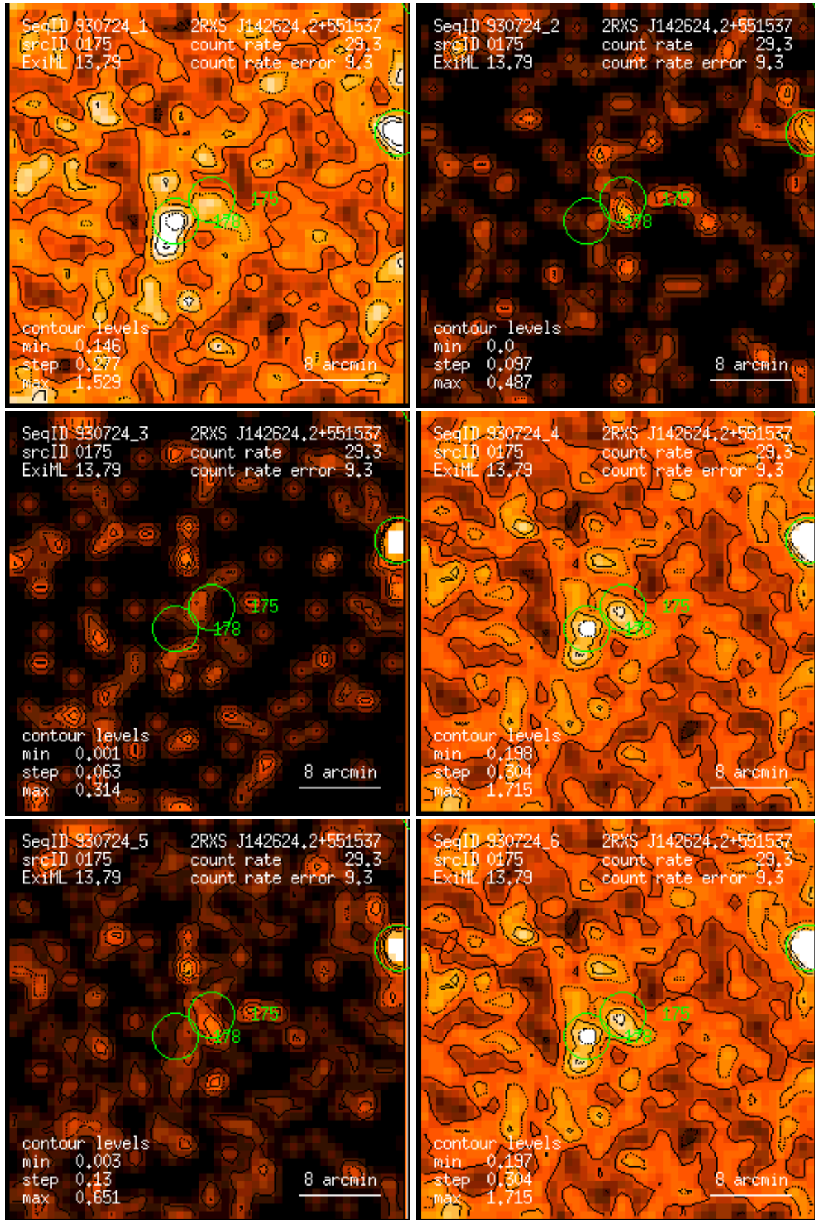
Figure 175: RASS 930724: detection 0175: band rate images, Gaussian filter: (1) PSPC channels 11 – 41, (2) 52 – 90, (3) 91 – 201, (4) 11 – 235, (5) 52 – 201, (6) 11 – 201. Broad band rates in counts/ks. Band rate contour levels in counts/ks/arcmin 2 .
