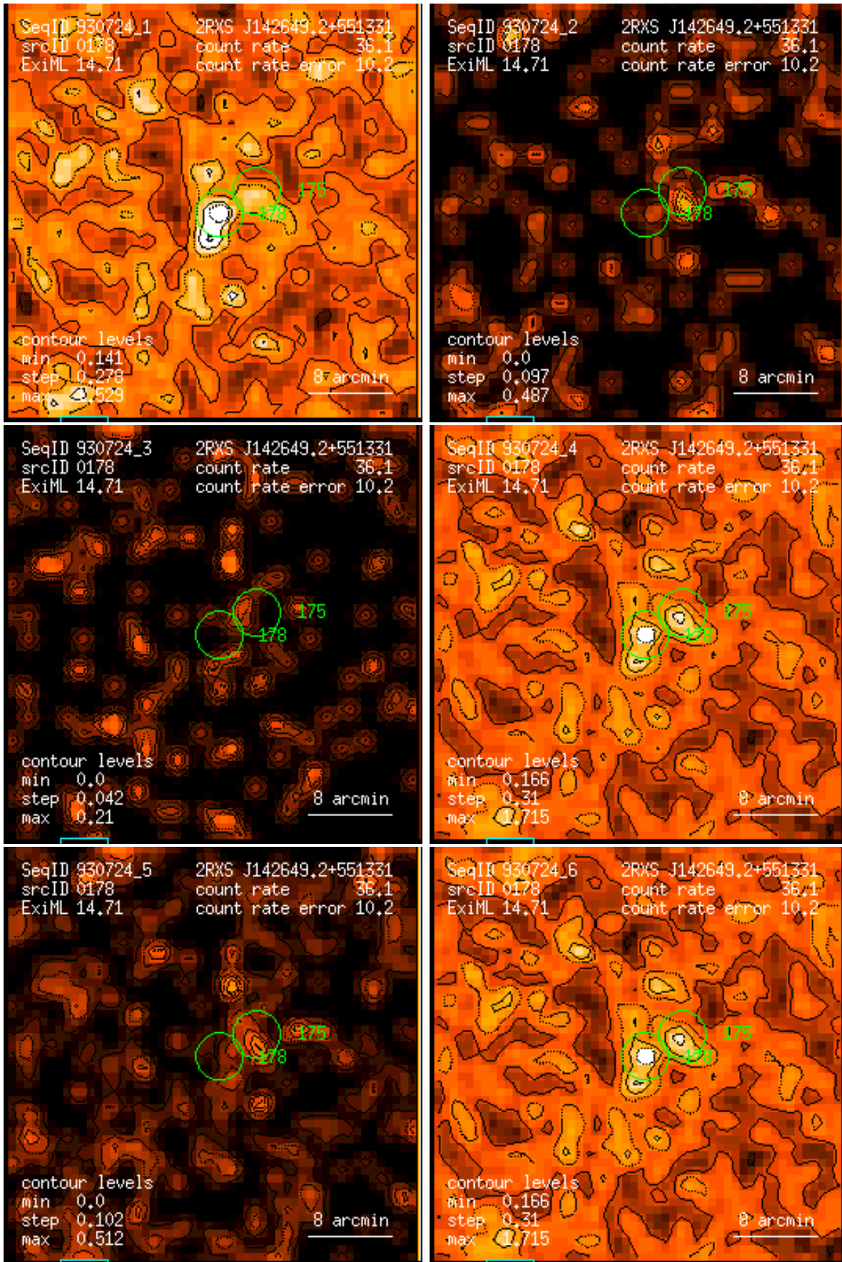
Figure 178: RASS 930724: detection 0178: band rate images, Gaussian filter: (1) PSPC channels 11 – 41, (2) 52 – 90, (3) 91 – 201, (4) 11 – 235, (5) 52 – 201, (6) 11 – 201. Broad band rates in counts/ks. Band rate contour levels in counts/ks/arcmin 2 .
