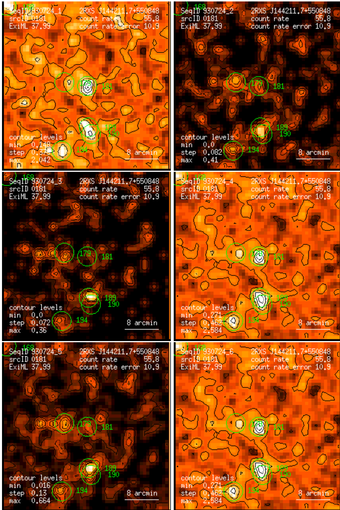
Figure 181: RASS 930724: detection 0181: band rate images, Gaussian filter: (1) PSPC channels 11 – 41, (2) 52 – 90, (3) 91 – 201, (4) 11 – 235, (5) 52 – 201, (6) 11 – 201. Broad band rates in counts/ks. Band rate contour levels in counts/ks/arcmin 2 .
