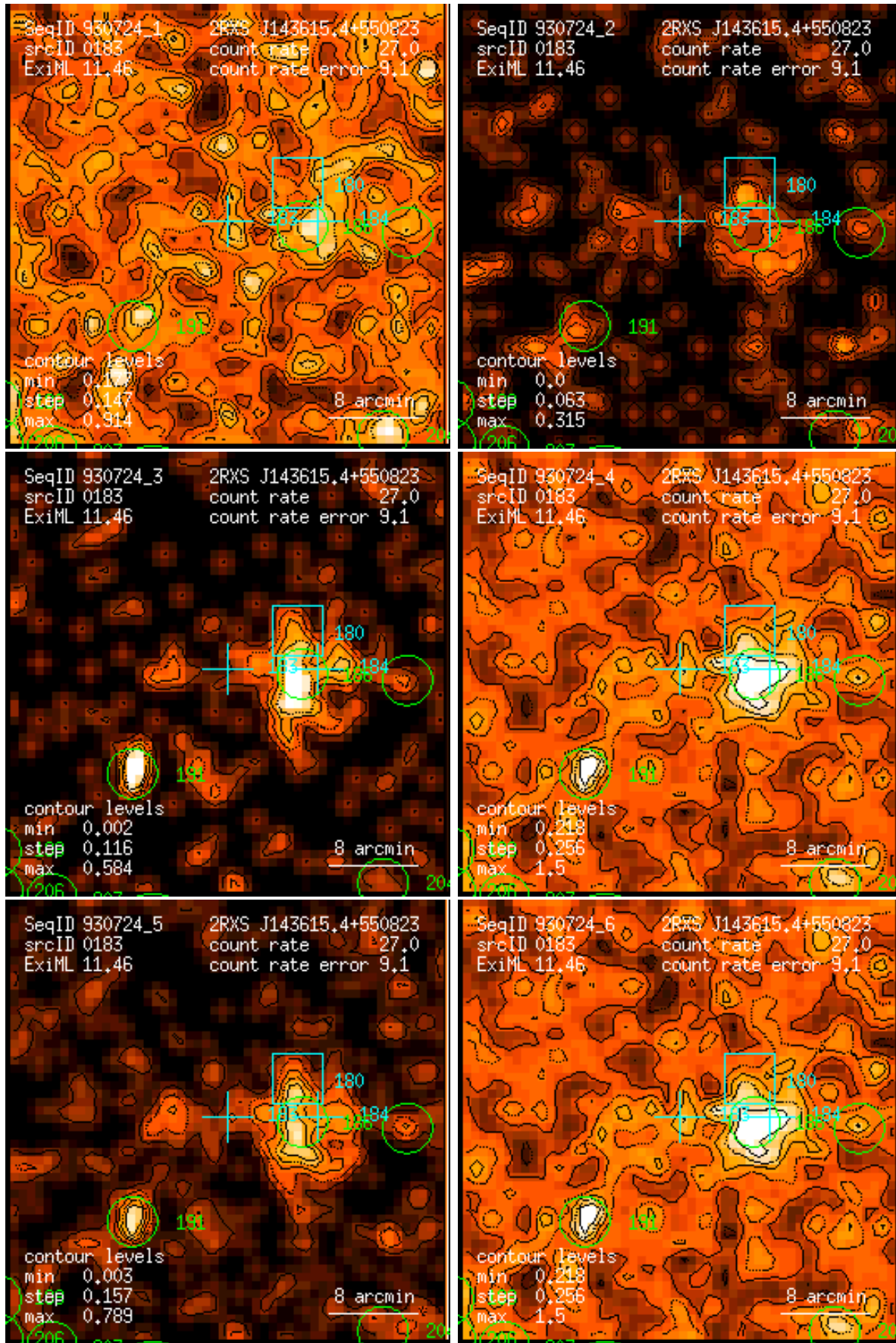
Figure 183: RASS 930724: detection 0183: band rate images, Gaussian filter: (1) PSPC channels 11 – 41, (2) 52 – 90, (3) 91 – 201, (4) 11 – 235, (5) 52 – 201, (6) 11 – 201. Broad band rates in counts/ks. Band rate contour levels in counts/ks/arcmin 2 .
