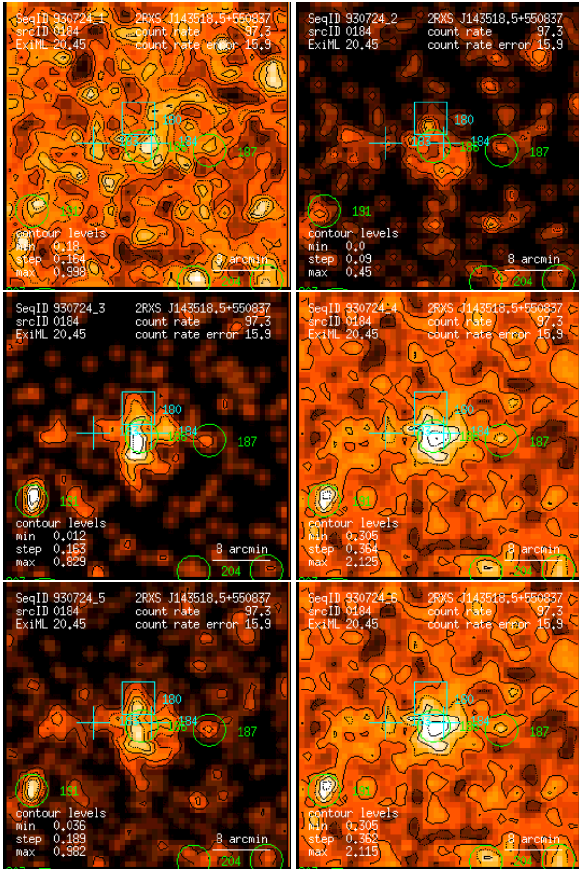
Figure 184: RASS 930724: detection 0184: band rate images, Gaussian filter: (1) PSPC channels 11 – 41, (2) 52 – 90, (3) 91 – 201, (4) 11 – 235, (5) 52 – 201, (6) 11 – 201. Broad band rates in counts/ks. Band rate contour levels in counts/ks/arcmin 2 .
