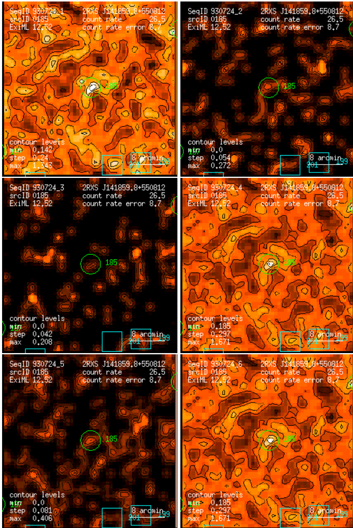
Figure 185: RASS 930724: detection 0185: band rate images, Gaussian filter: (1) PSPC channels 11 – 41, (2) 52 – 90, (3) 91 – 201, (4) 11 – 235, (5) 52 – 201, (6) 11 – 201. Broad band rates in counts/ks. Band rate contour levels in counts/ks/arcmin 2 .
