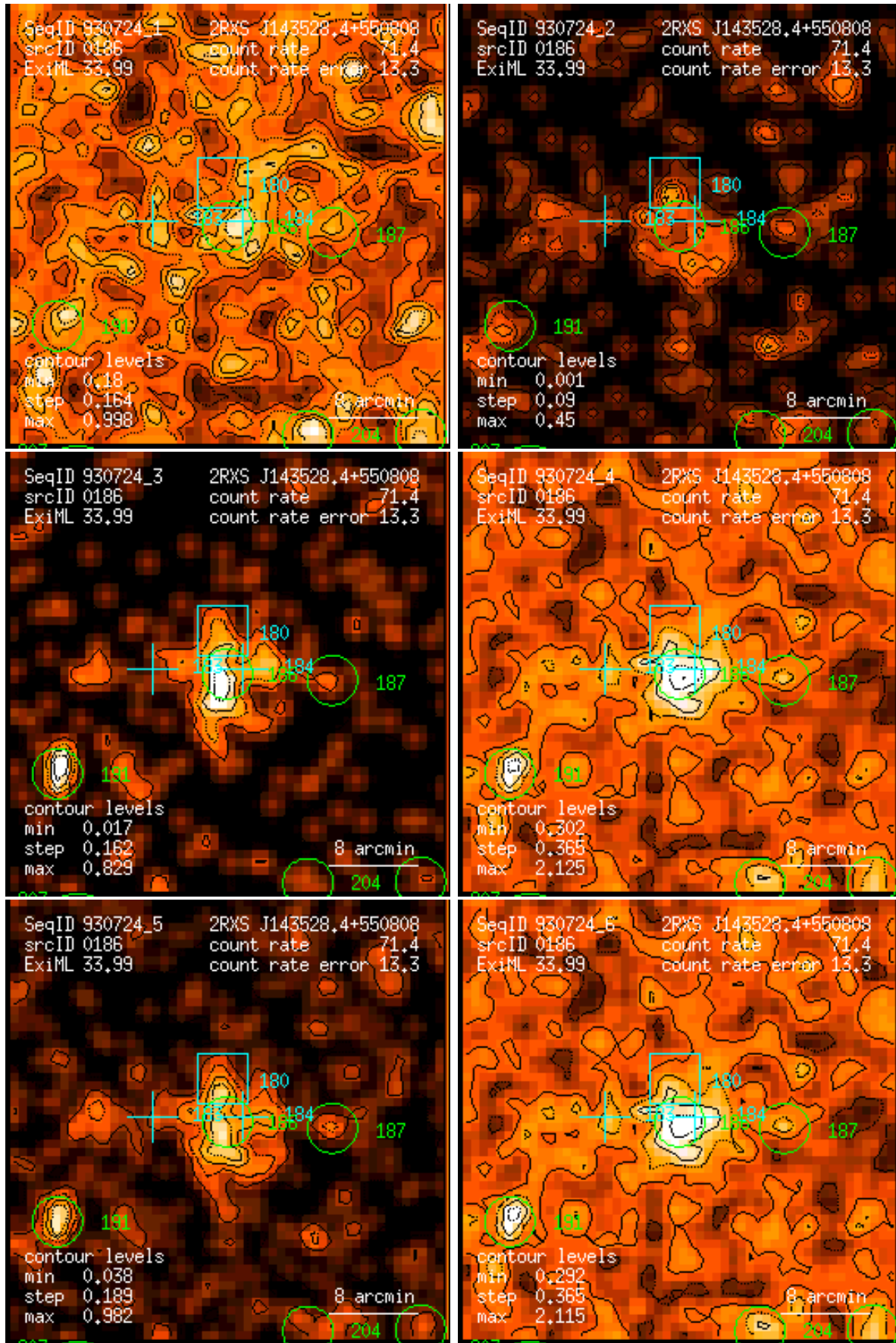
Figure 186: RASS 930724: detection 0186: band rate images, Gaussian filter: (1) PSPC channels 11 – 41, (2) 52 – 90, (3) 91 – 201, (4) 11 – 235, (5) 52 – 201, (6) 11 – 201. Broad band rates in counts/ks. Band rate contour levels in counts/ks/arcmin 2 .
