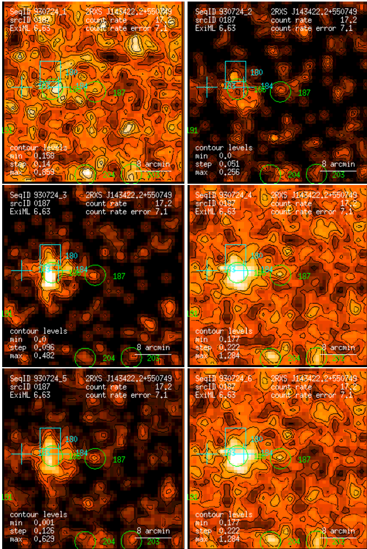
Figure 187: RASS 930724: detection 0187: band rate images, Gaussian filter: (1) PSPC channels 11 – 41, (2) 52 – 90, (3) 91 – 201, (4) 11 – 235, (5) 52 – 201, (6) 11 – 201. Broad band rates in counts/ks. Band rate contour levels in counts/ks/arcmin 2 .
