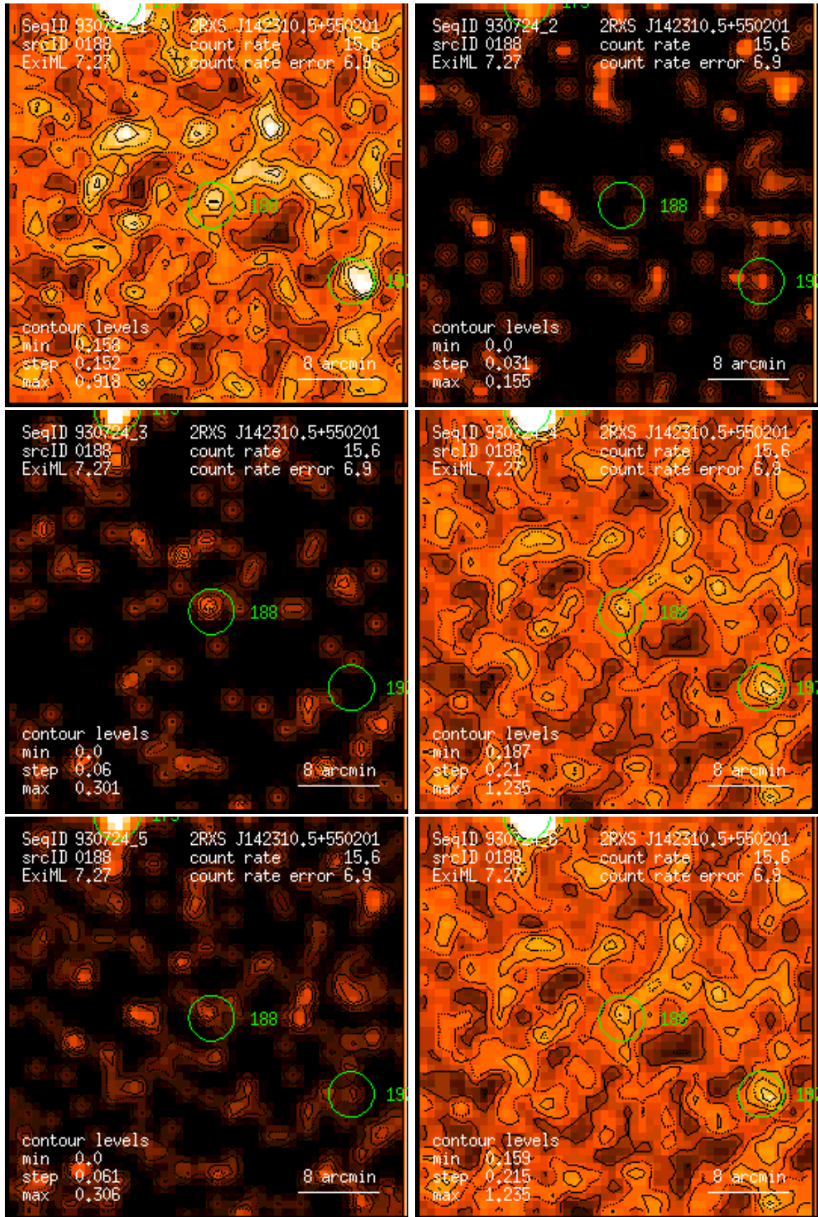
Figure 188: RASS 930724: detection 0188: band rate images, Gaussian filter: (1) PSPC channels 11 – 41, (2) 52 – 90, (3) 91 – 201, (4) 11 – 235, (5) 52 – 201, (6) 11 – 201. Broad band rates in counts/ks. Band rate contour levels in counts/ks/arcmin 2 .
