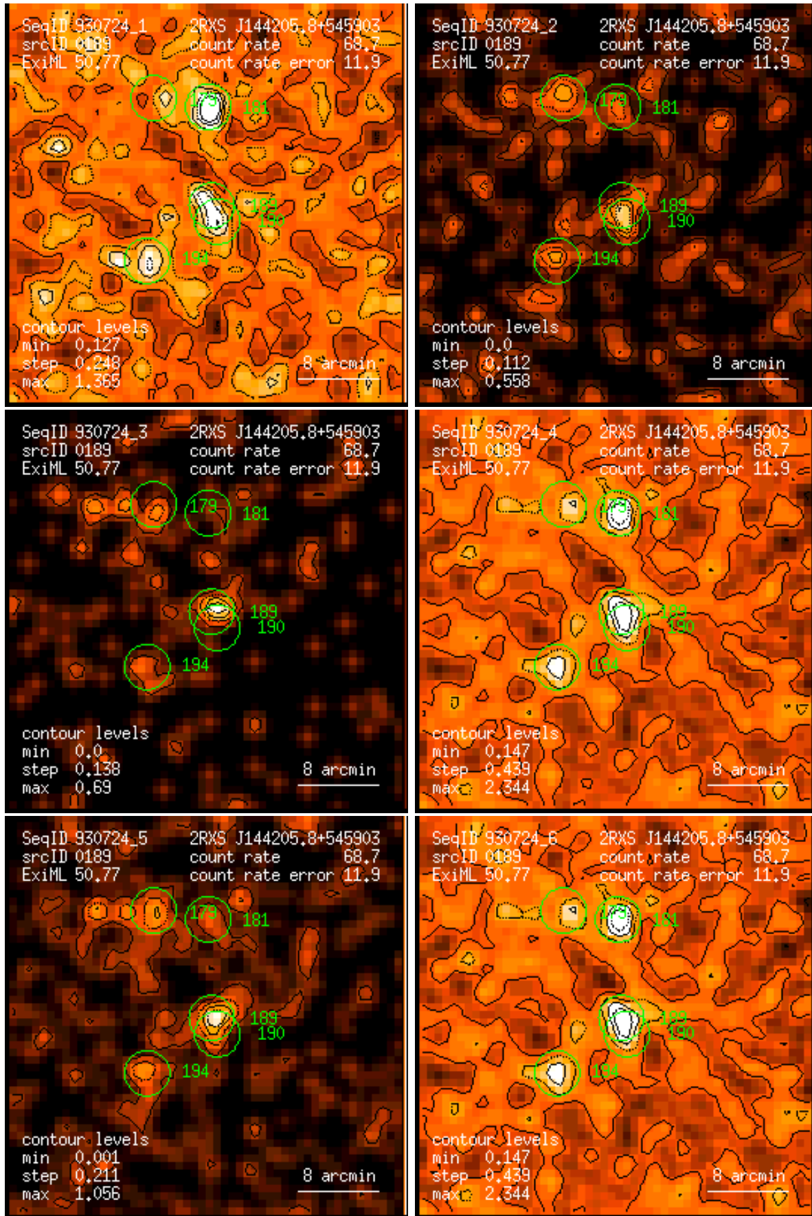
Figure 189: RASS 930724: detection 0189: band rate images, Gaussian filter: (1) PSPC channels 11 – 41, (2) 52 – 90, (3) 91 – 201, (4) 11 – 235, (5) 52 – 201, (6) 11 – 201. Broad band rates in counts/ks. Band rate contour levels in counts/ks/arcmin 2 .
