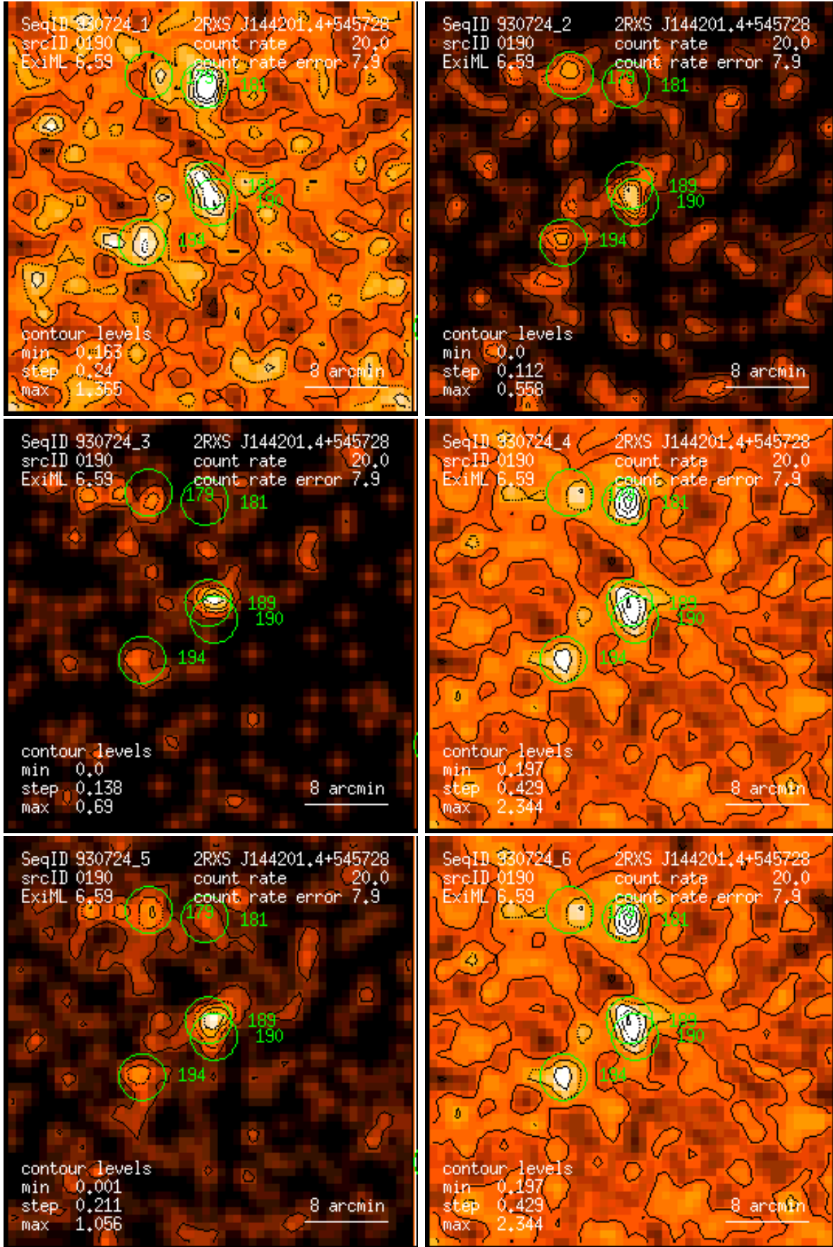
Figure 190: RASS 930724: detection 0190: band rate images, Gaussian filter: (1) PSPC channels 11 – 41, (2) 52 – 90, (3) 91 – 201, (4) 11 – 235, (5) 52 – 201, (6) 11 – 201. Broad band rates in counts/ks. Band rate contour levels in counts/ks/arcmin 2 .
