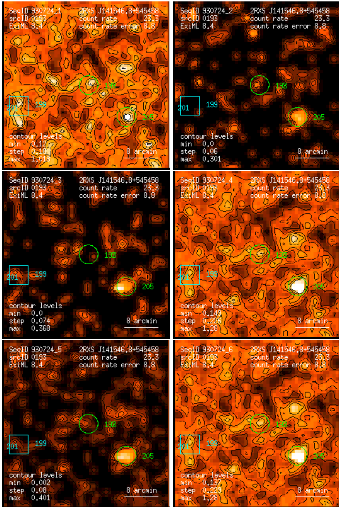
Figure 193: RASS 930724: detection 0193: band rate images, Gaussian filter: (1) PSPC channels 11 – 41, (2) 52 – 90, (3) 91 – 201, (4) 11 – 235, (5) 52 – 201, (6) 11 – 201. Broad band rates in counts/ks. Band rate contour levels in counts/ks/arcmin 2 .
