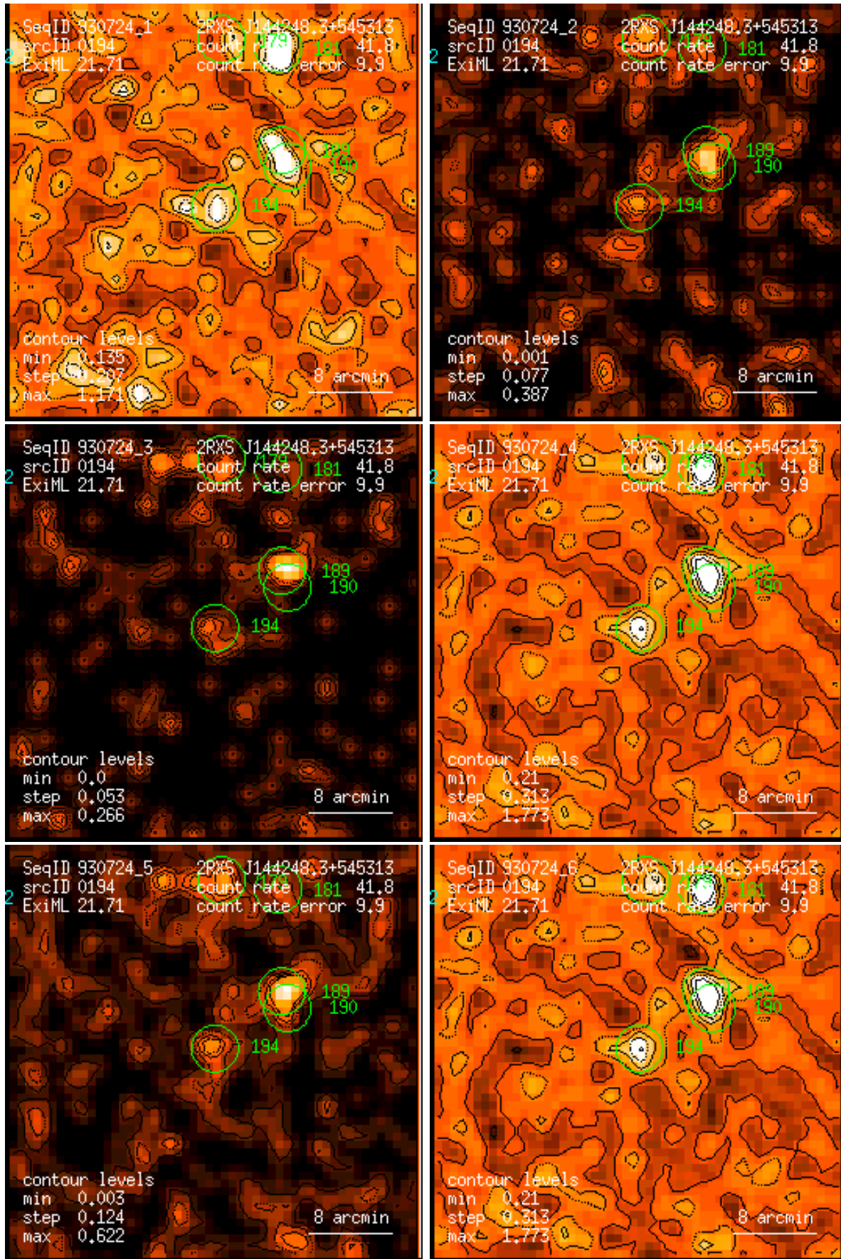
Figure 194: RASS 930724: detection 0194: band rate images, Gaussian filter: (1) PSPC channels 11 – 41, (2) 52 – 90, (3) 91 – 201, (4) 11 – 235, (5) 52 – 201, (6) 11 – 201. Broad band rates in counts/ks. Band rate contour levels in counts/ks/arcmin 2 .
