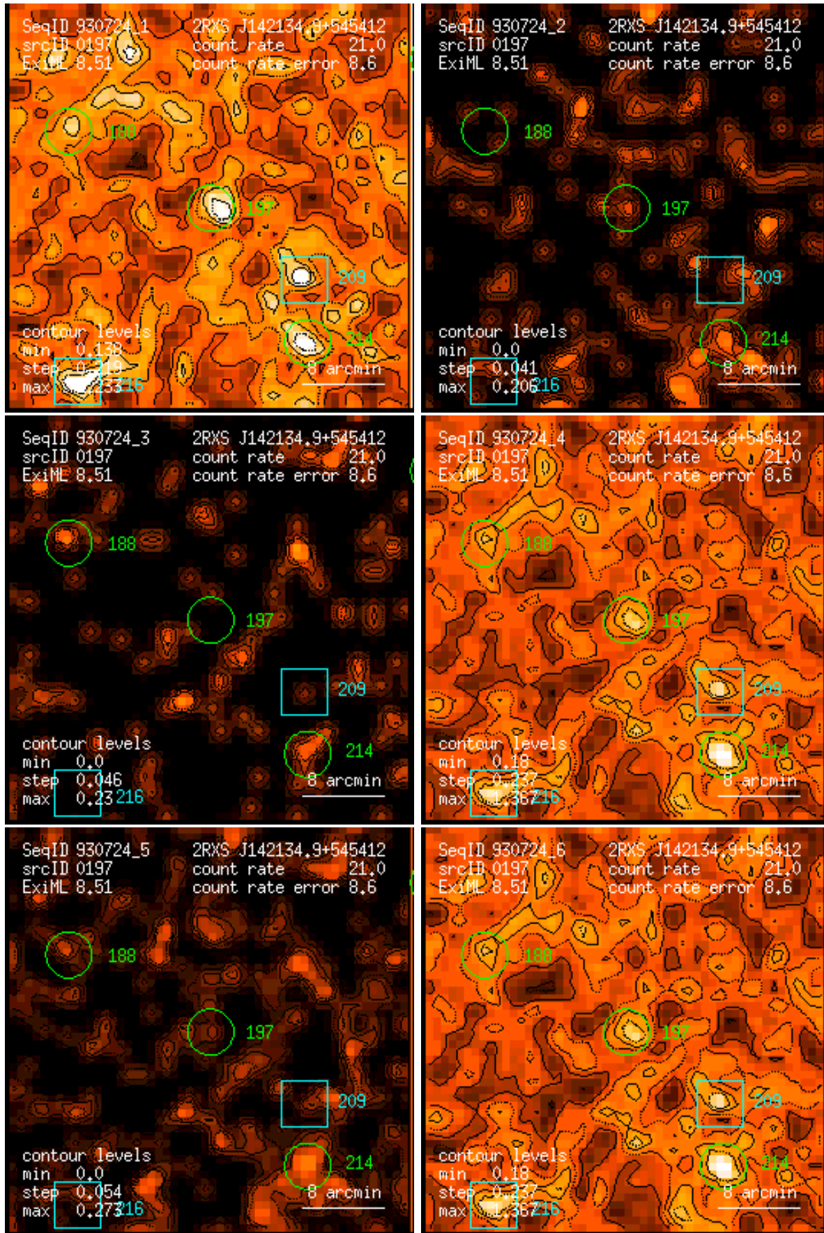
Figure 197: RASS 930724: detection 0197: band rate images, Gaussian filter: (1) PSPC channels 11 – 41, (2) 52 – 90, (3) 91 – 201, (4) 11 – 235, (5) 52 – 201, (6) 11 – 201. Broad band rates in counts/ks. Band rate contour levels in counts/ks/arcmin 2 .
