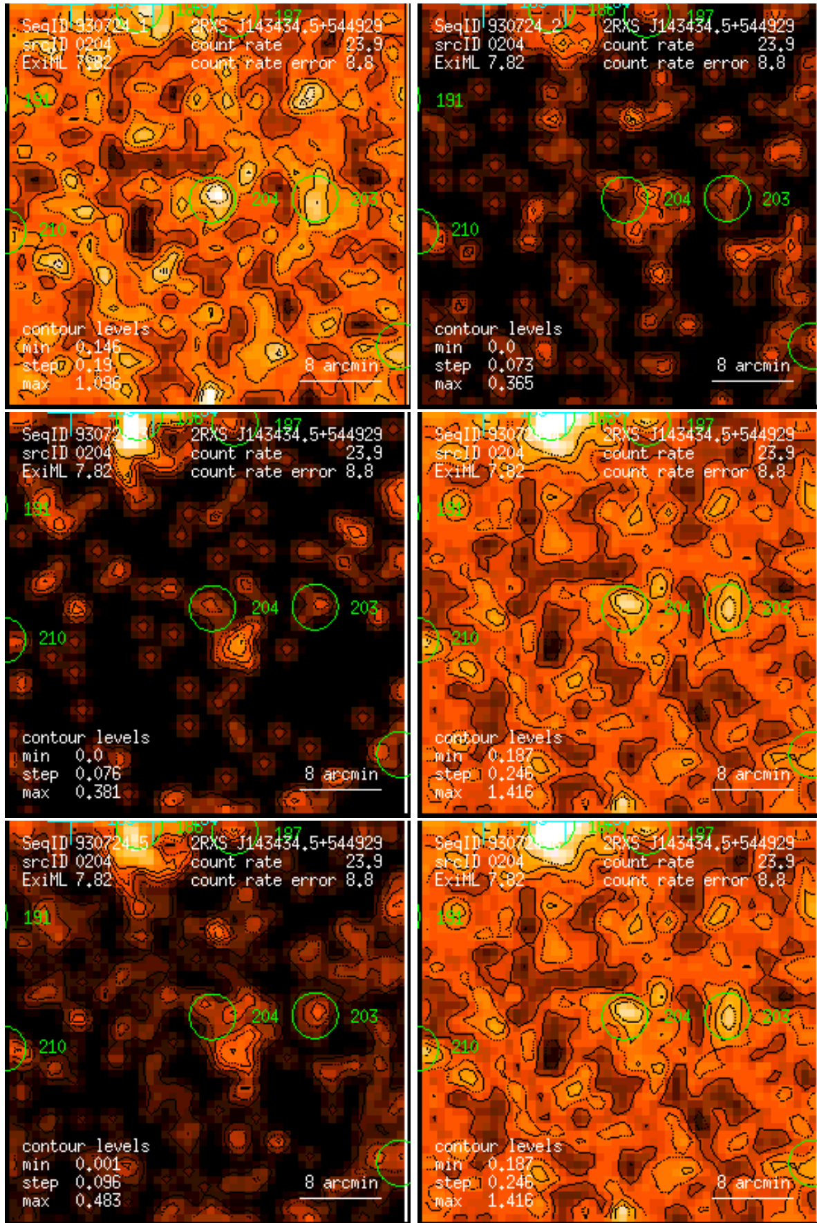
Figure 204: RASS 930724: detection 0204: band rate images, Gaussian filter: (1) PSPC channels 11 – 41, (2) 52 – 90, (3) 91 – 201, (4) 11 – 235, (5) 52 – 201, (6) 11 – 201. Broad band rates in counts/ks. Band rate contour levels in counts/ks/arcmin 2 .
