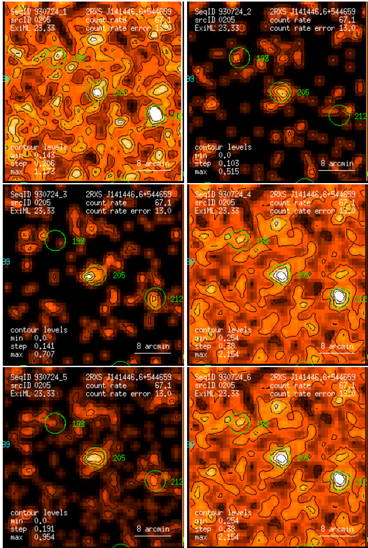
Figure 205: RASS 930724: detection 0205: band rate images, Gaussian filter: (1) PSPC channels 11 – 41, (2) 52 – 90, (3) 91 – 201, (4) 11 – 235, (5) 52 – 201, (6) 11 – 201. Broad band rates in counts/ks. Band rate contour levels in counts/ks/arcmin 2 .
