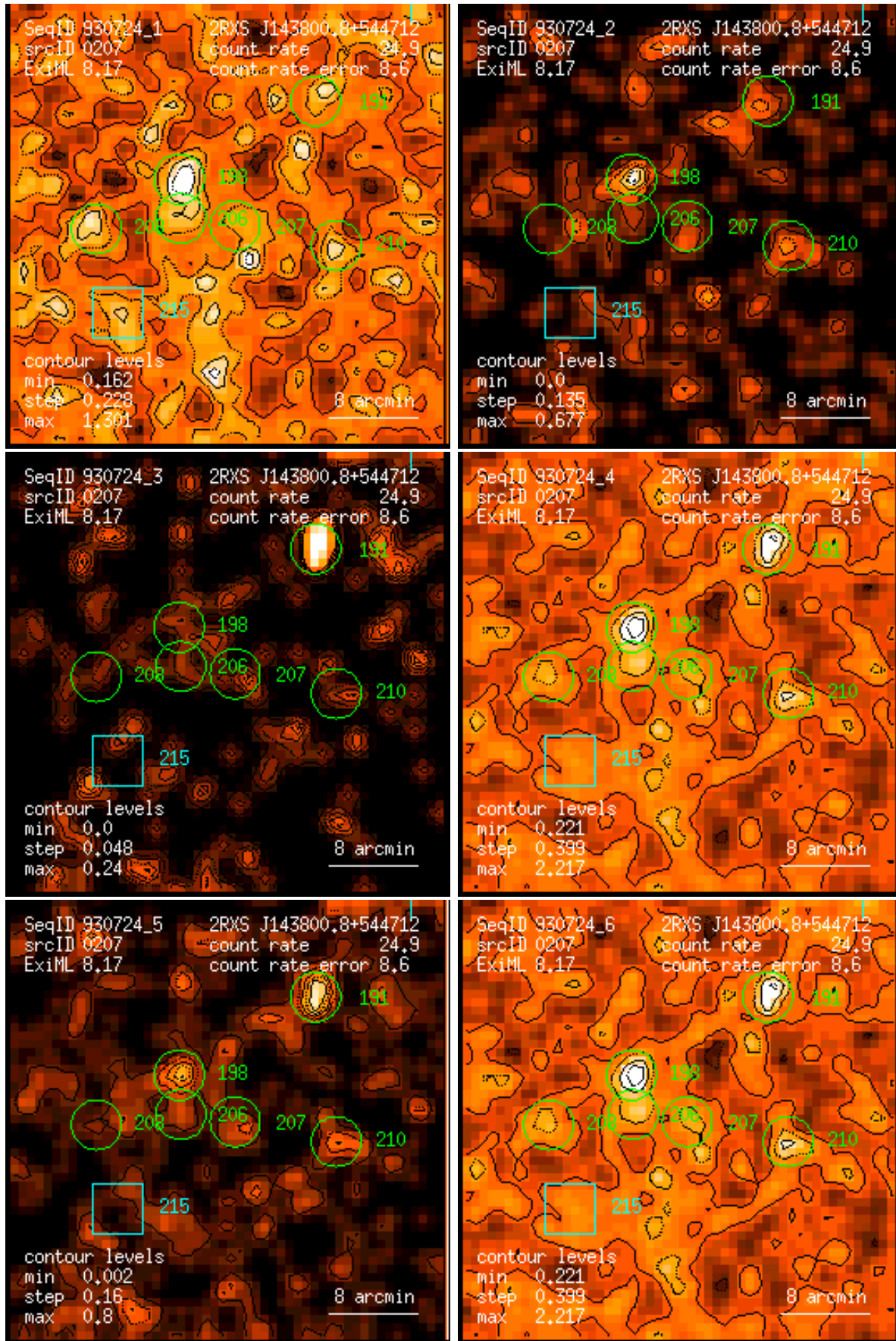
Figure 207: RASS 930724: detection 0207: band rate images, Gaussian filter: (1) PSPC channels 11 – 41, (2) 52 – 90, (3) 91 – 201, (4) 11 – 235, (5) 52 – 201, (6) 11 – 201. Broad band rates in counts/ks. Band rate contour levels in counts/ks/arcmin 2 .
