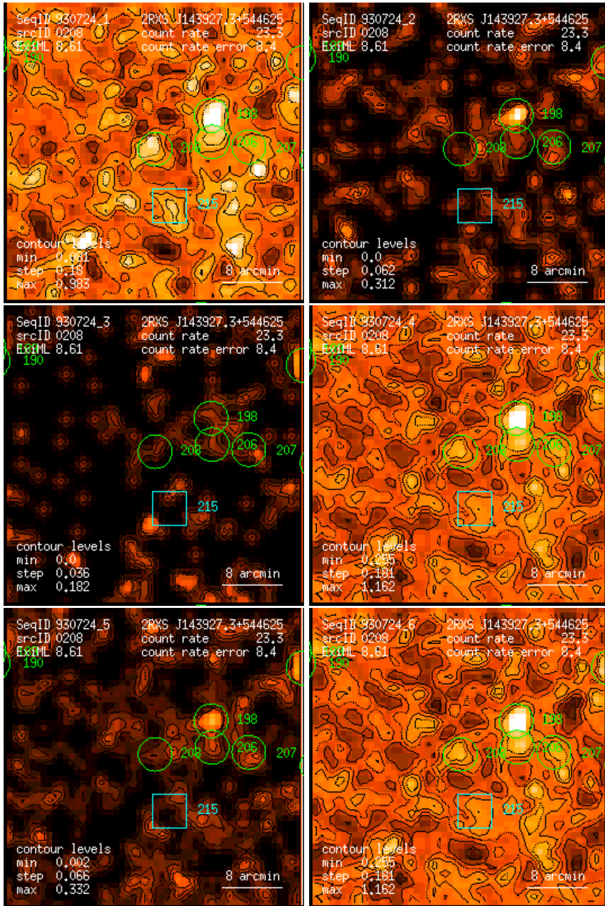
Figure 208: RASS 930724: detection 0208: band rate images, Gaussian filter: (1) PSPC channels 11 – 41, (2) 52 – 90, (3) 91 – 201, (4) 11 – 235, (5) 52 – 201, (6) 11 – 201. Broad band rates in counts/ks. Band rate contour levels in counts/ks/arcmin 2 .
