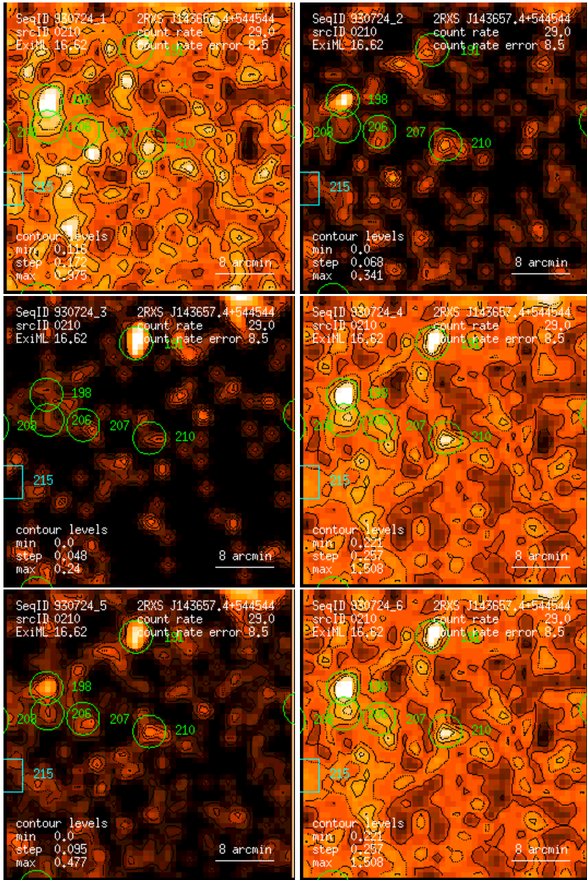
Figure 210: RASS 930724: detection 0210: band rate images, Gaussian filter: (1) PSPC channels 11 – 41, (2) 52 – 90, (3) 91 – 201, (4) 11 – 235, (5) 52 – 201, (6) 11 – 201. Broad band rates in counts/ks. Band rate contour levels in counts/ks/arcmin 2 .
