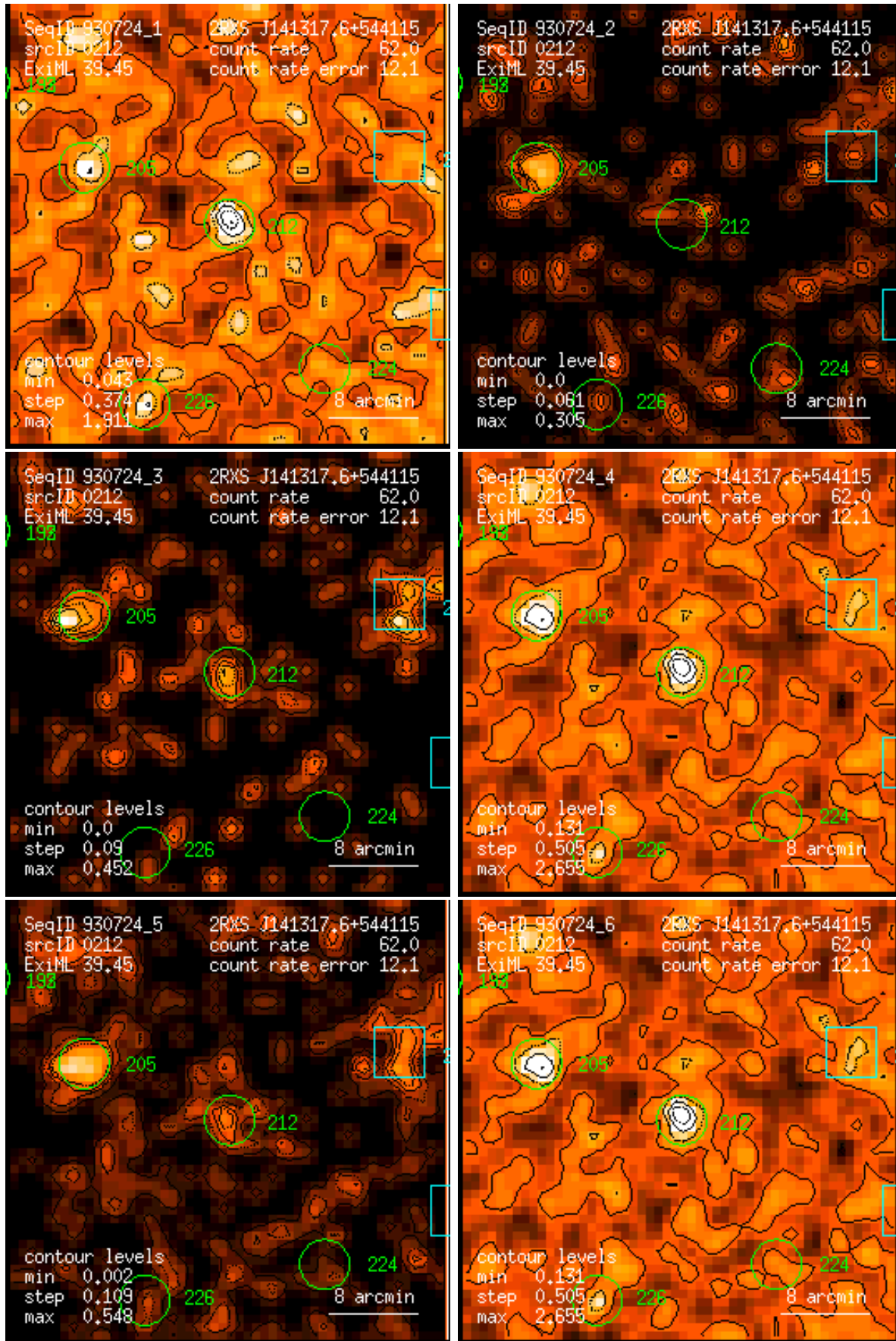
Figure 212: RASS 930724: detection 0212: band rate images, Gaussian filter: (1) PSPC channels 11 – 41, (2) 52 – 90, (3) 91 – 201, (4) 11 – 235, (5) 52 – 201, (6) 11 – 201. Broad band rates in counts/ks. Band rate contour levels in counts/ks/arcmin 2 .
