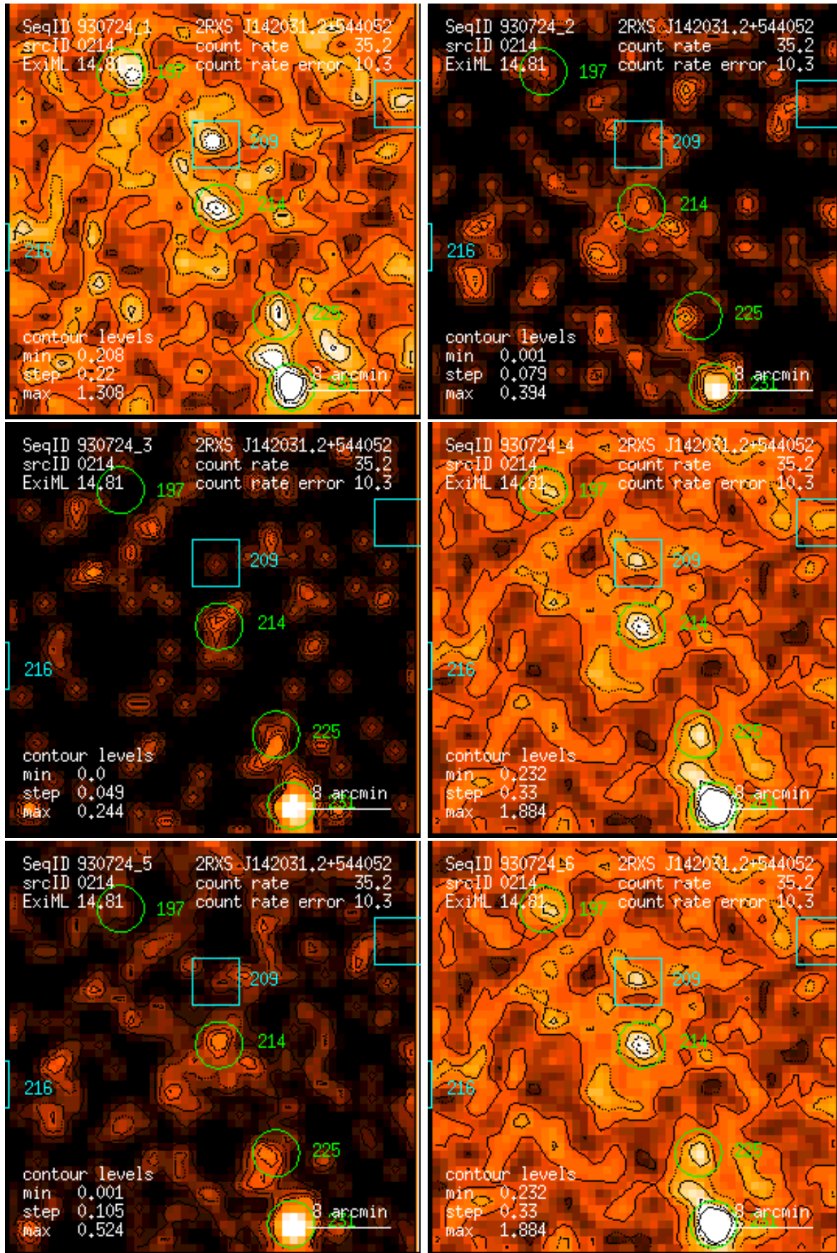
Figure 214: RASS 930724: detection 0214: band rate images, Gaussian filter: (1) PSPC channels 11 – 41, (2) 52 – 90, (3) 91 – 201, (4) 11 – 235, (5) 52 – 201, (6) 11 – 201. Broad band rates in counts/ks. Band rate contour levels in counts/ks/arcmin 2 .
