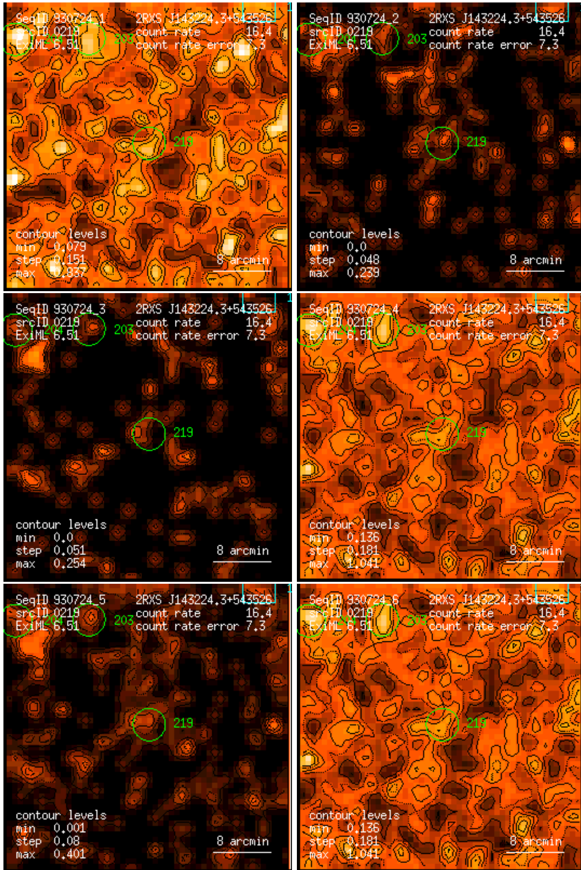
Figure 219: RASS 930724: detection 0219: band rate images, Gaussian filter: (1) PSPC channels 11 – 41, (2) 52 – 90, (3) 91 – 201, (4) 11 – 235, (5) 52 – 201, (6) 11 – 201. Broad band rates in counts/ks. Band rate contour levels in counts/ks/arcmin 2 .
