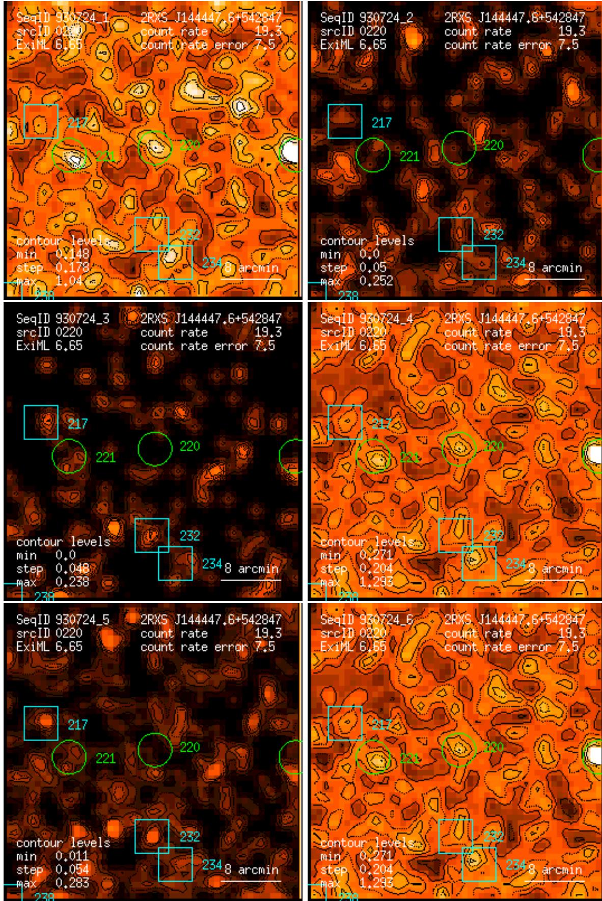
Figure 220: RASS 930724: detection 0220: band rate images, Gaussian filter: (1) PSPC channels 11 – 41, (2) 52 – 90, (3) 91 – 201, (4) 11 – 235, (5) 52 – 201, (6) 11 – 201. Broad band rates in counts/ks. Band rate contour levels in counts/ks/arcmin 2 .
