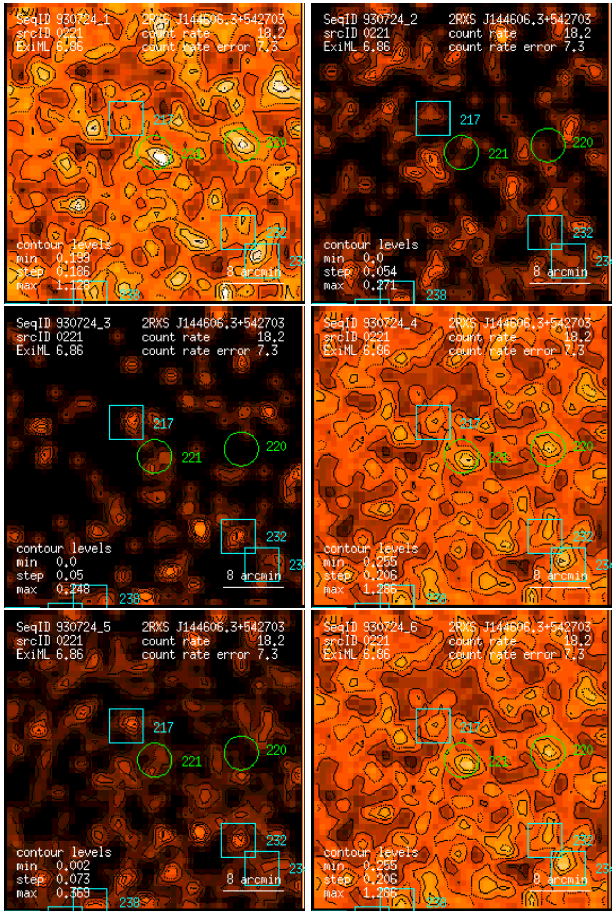
Figure 221: RASS 930724: detection 0221: band rate images, Gaussian filter: (1) PSPC channels 11 – 41, (2) 52 – 90, (3) 91 – 201, (4) 11 – 235, (5) 52 – 201, (6) 11 – 201. Broad band rates in counts/ks. Band rate contour levels in counts/ks/arcmin 2 .
