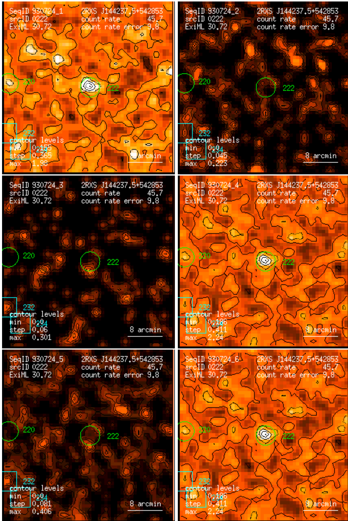
Figure 222: RASS 930724: detection 0222: band rate images, Gaussian filter: (1) PSPC channels 11 – 41, (2) 52 – 90, (3) 91 – 201, (4) 11 – 235, (5) 52 – 201, (6) 11 – 201. Broad band rates in counts/ks. Band rate contour levels in counts/ks/arcmin 2 .
