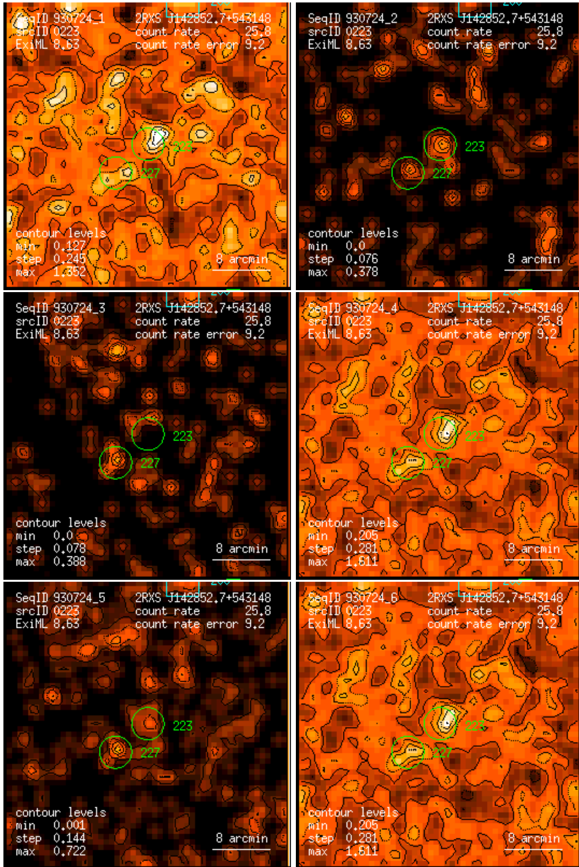
Figure 223: RASS 930724: detection 0223: band rate images, Gaussian filter: (1) PSPC channels 11 – 41, (2) 52 – 90, (3) 91 – 201, (4) 11 – 235, (5) 52 – 201, (6) 11 – 201. Broad band rates in counts/ks. Band rate contour levels in counts/ks/arcmin 2 .
