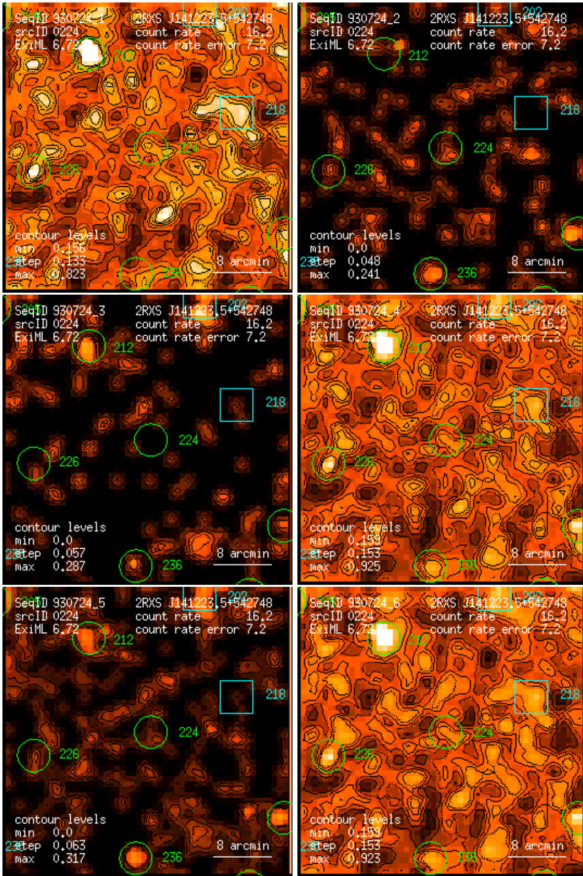
Figure 224: RASS 930724: detection 0224: band rate images, Gaussian filter: (1) PSPC channels 11 – 41, (2) 52 – 90, (3) 91 – 201, (4) 11 – 235, (5) 52 – 201, (6) 11 – 201. Broad band rates in counts/ks. Band rate contour levels in counts/ks/arcmin 2 .
