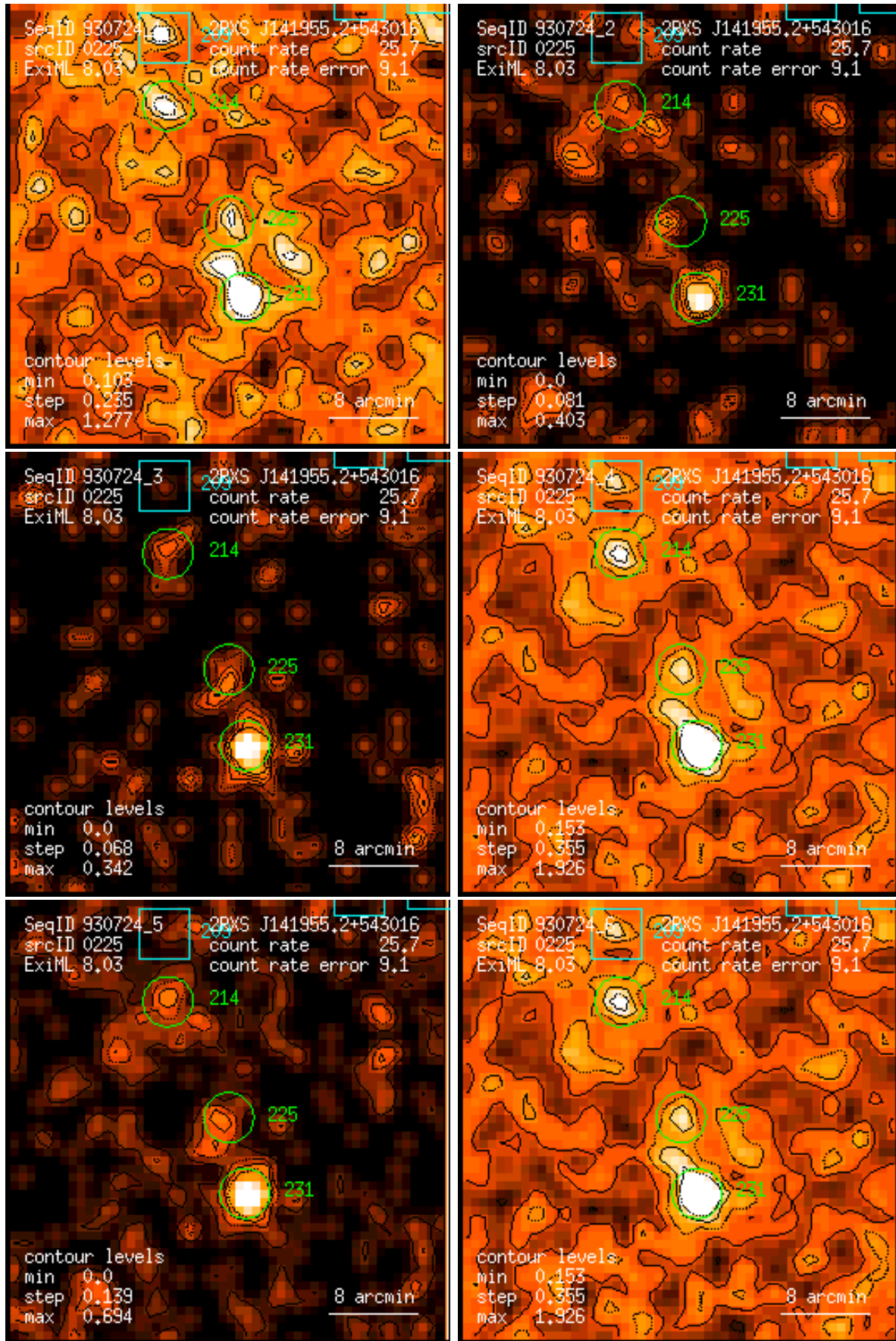
Figure 225: RASS 930724: detection 0225: band rate images, Gaussian filter: (1) PSPC channels 11 – 41, (2) 52 – 90, (3) 91 – 201, (4) 11 – 235, (5) 52 – 201, (6) 11 – 201. Broad band rates in counts/ks. Band rate contour levels in counts/ks/arcmin 2 .
