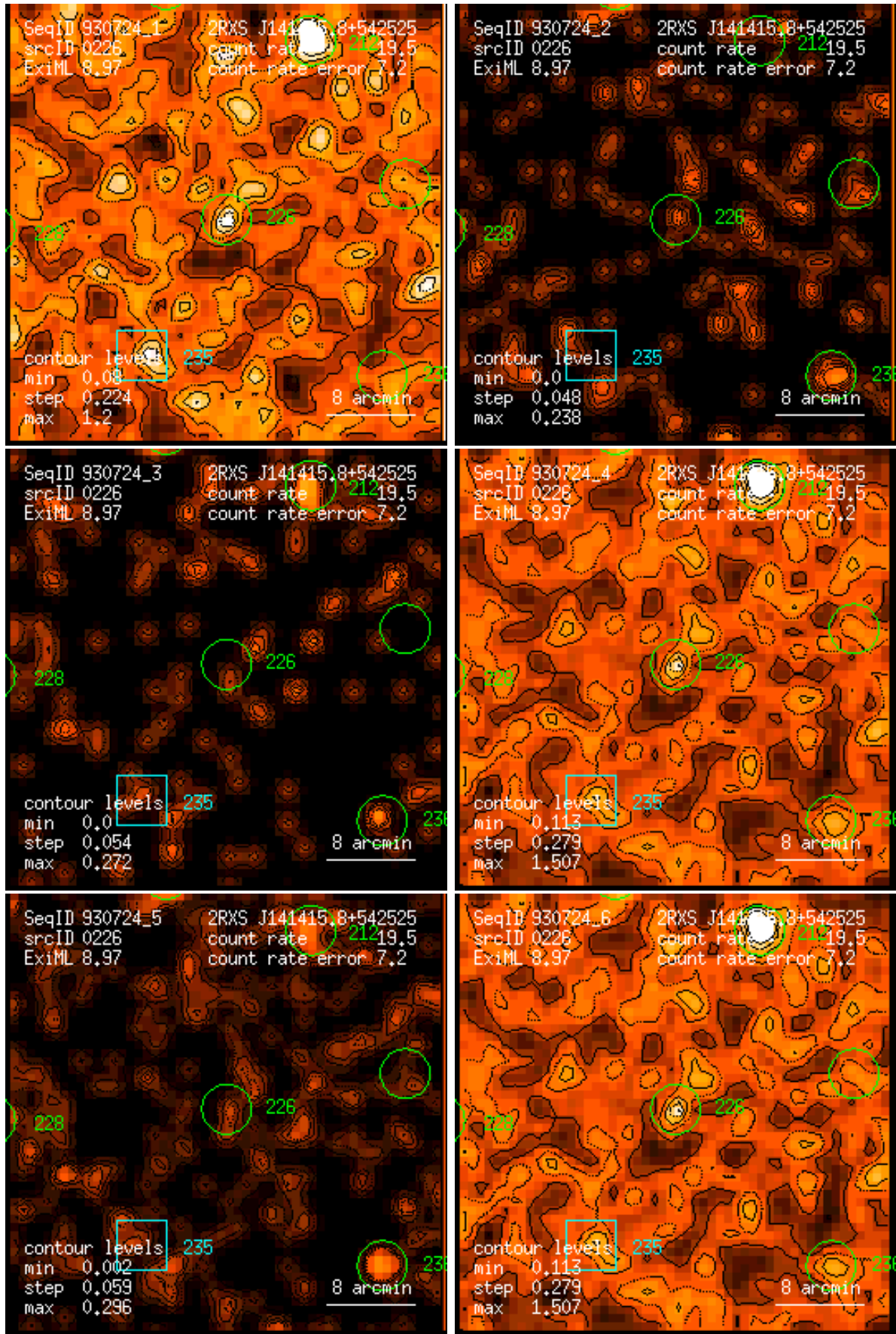
Figure 226: RASS 930724: detection 0226: band rate images, Gaussian filter: (1) PSPC channels 11 – 41, (2) 52 – 90, (3) 91 – 201, (4) 11 – 235, (5) 52 – 201, (6) 11 – 201. Broad band rates in counts/ks. Band rate contour levels in counts/ks/arcmin 2 .
