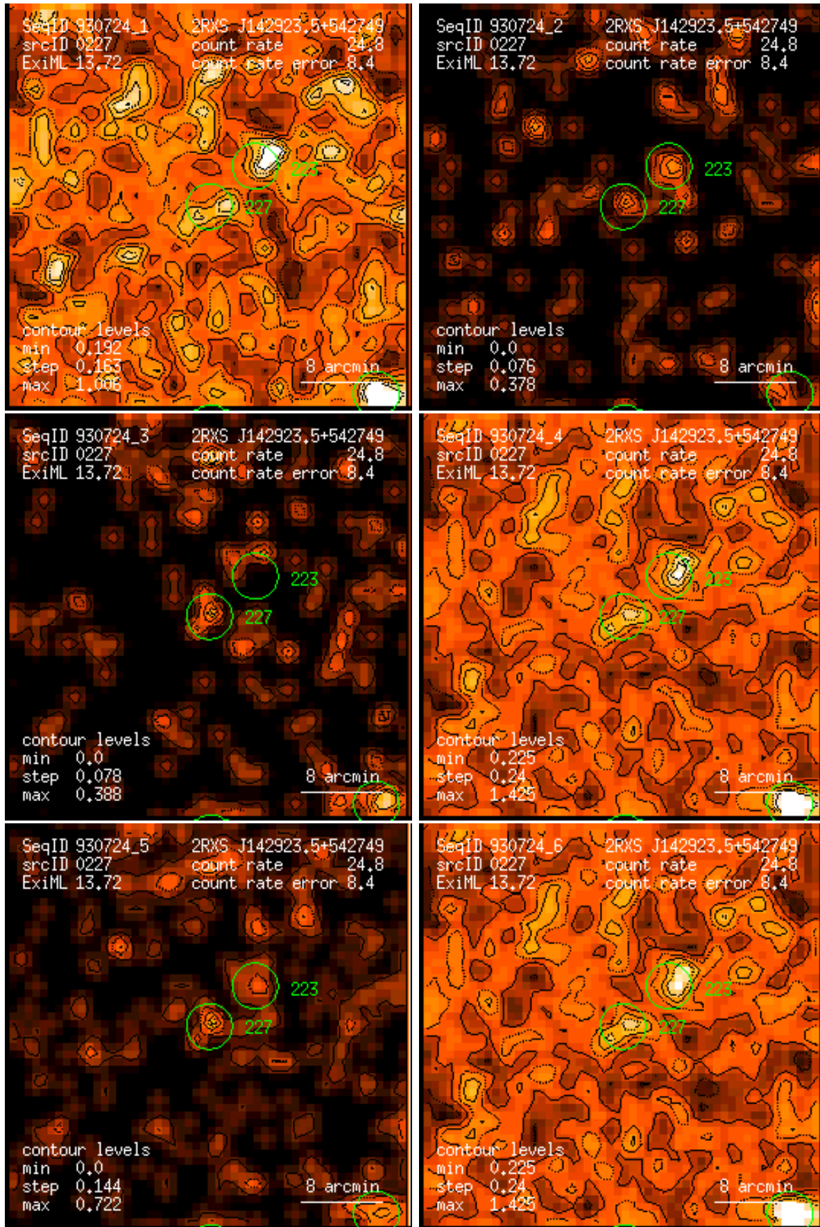
Figure 227: RASS 930724: detection 0227: band rate images, Gaussian filter: (1) PSPC channels 11 – 41, (2) 52 – 90, (3) 91 – 201, (4) 11 – 235, (5) 52 – 201, (6) 11 – 201. Broad band rates in counts/ks. Band rate contour levels in counts/ks/arcmin 2 .
