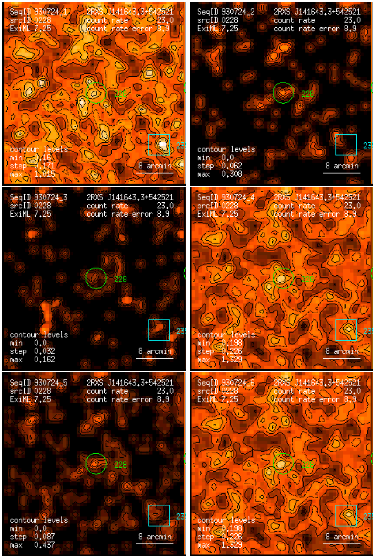
Figure 228: RASS 930724: detection 0228: band rate images, Gaussian filter: (1) PSPC channels 11 – 41, (2) 52 – 90, (3) 91 – 201, (4) 11 – 235, (5) 52 – 201, (6) 11 – 201. Broad band rates in counts/ks. Band rate contour levels in counts/ks/arcmin 2 .
