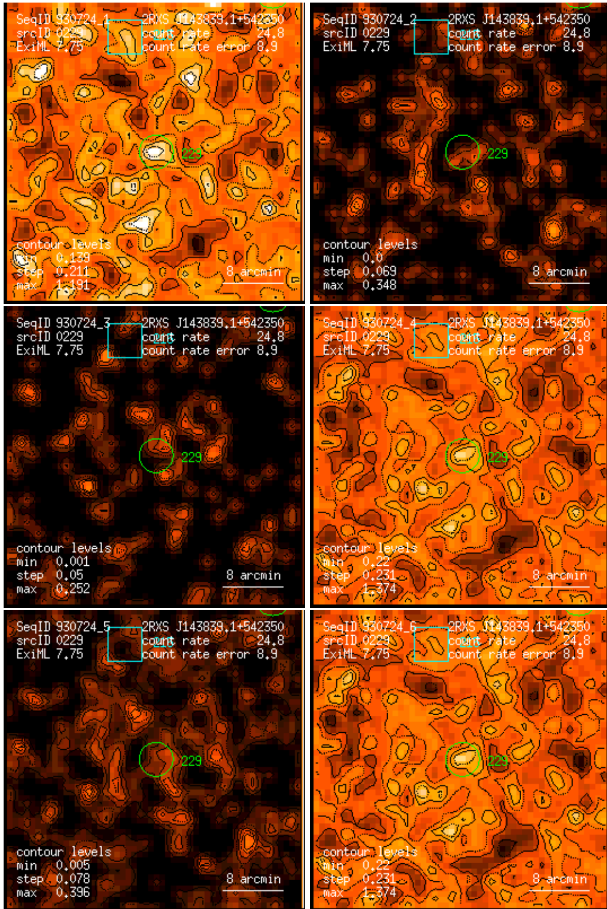
Figure 229: RASS 930724: detection 0229: band rate images, Gaussian filter: (1) PSPC channels 11 – 41, (2) 52 – 90, (3) 91 – 201, (4) 11 – 235, (5) 52 – 201, (6) 11 – 201. Broad band rates in counts/ks. Band rate contour levels in counts/ks/arcmin 2 .
