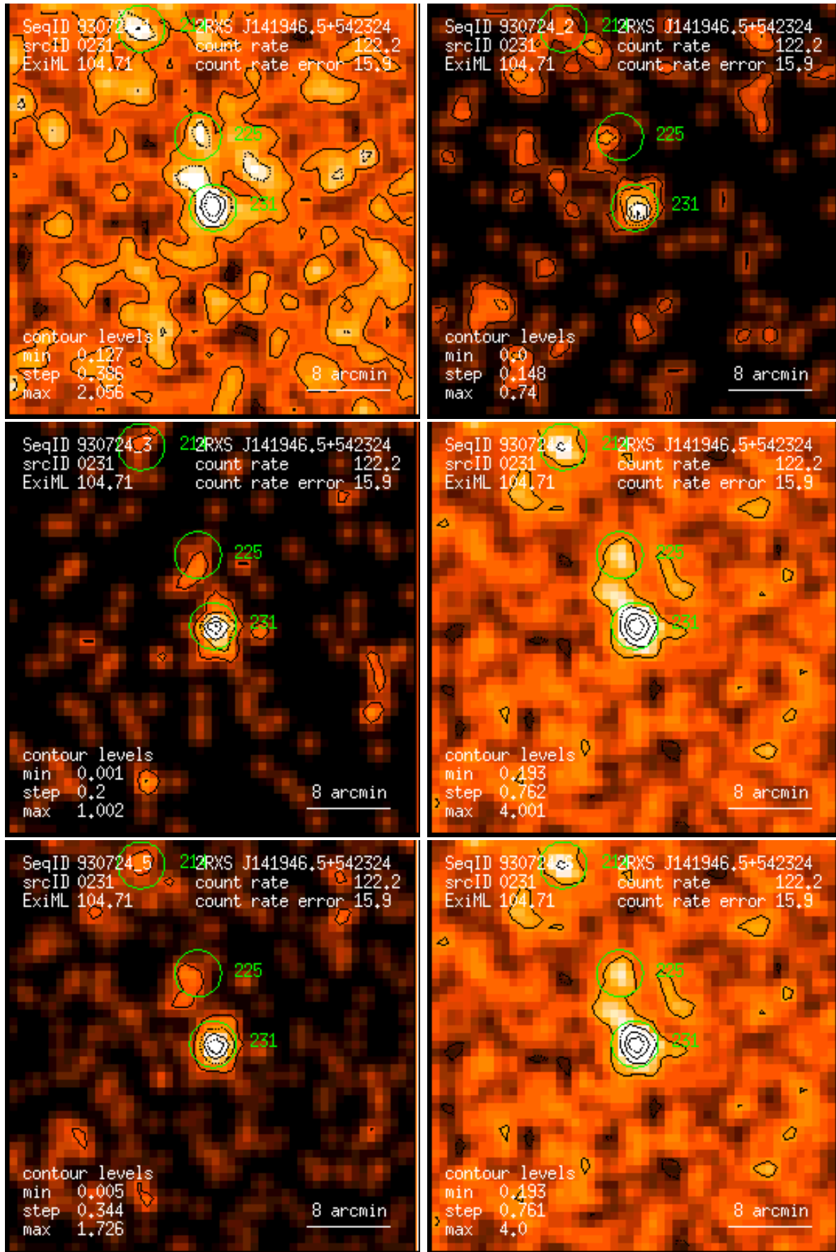
Figure 231: RASS 930724: detection 0231: band rate images, Gaussian filter: (1) PSPC channels 11 – 41, (2) 52 – 90, (3) 91 – 201, (4) 11 – 235, (5) 52 – 201, (6) 11 – 201. Broad band rates in counts/ks. Band rate contour levels in counts/ks/arcmin 2 .
