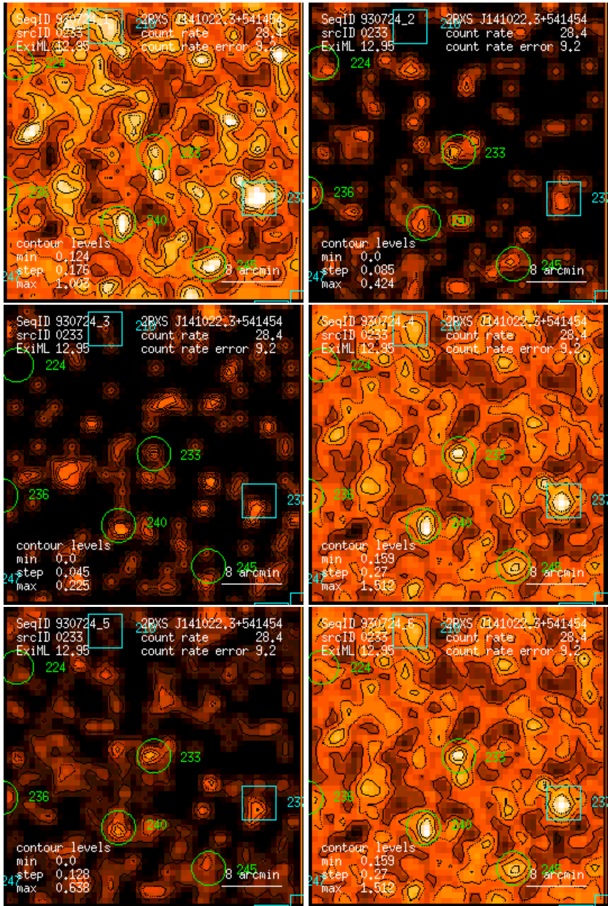
Figure 233: RASS 930724: detection 0233: band rate images, Gaussian filter: (1) PSPC channels 11 – 41, (2) 52 – 90, (3) 91 – 201, (4) 11 – 235, (5) 52 – 201, (6) 11 – 201. Broad band rates in counts/ks. Band rate contour levels in counts/ks/arcmin 2 .
