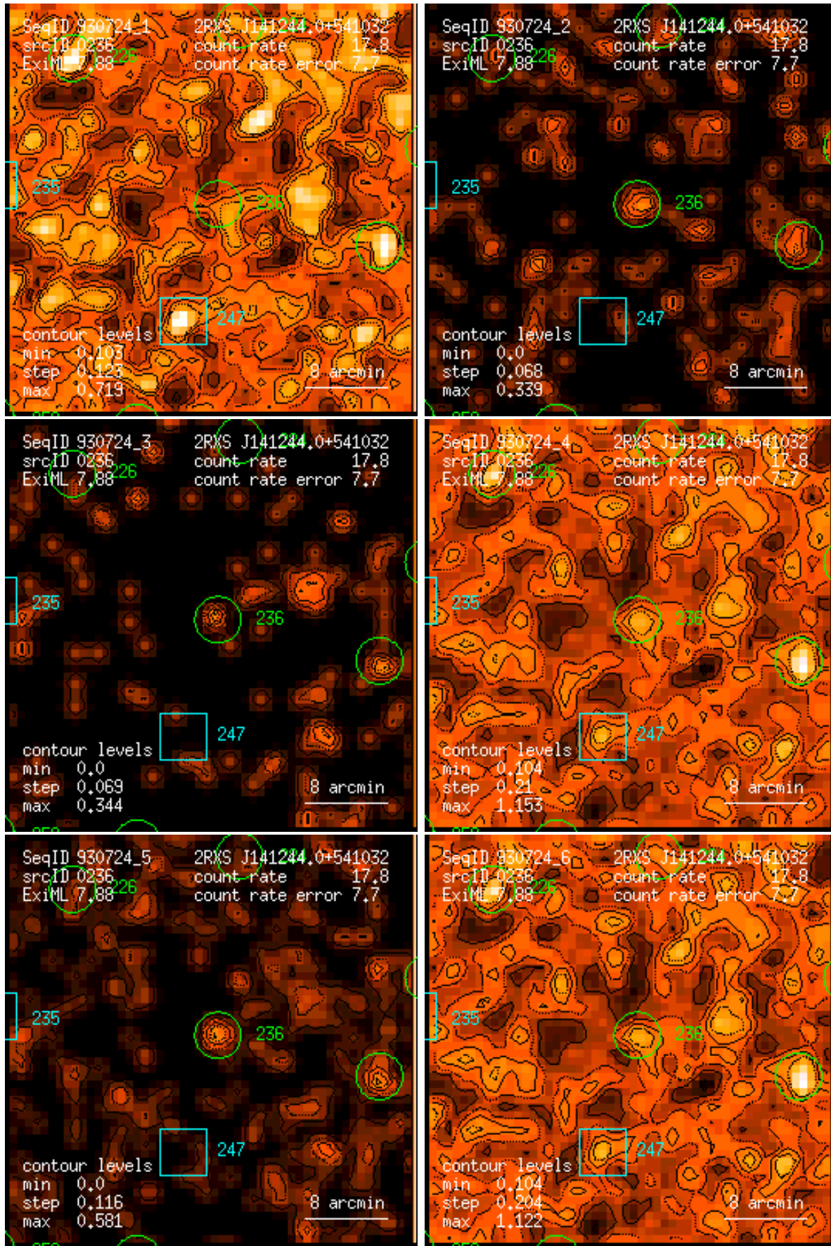
Figure 236: RASS 930724: detection 0236: band rate images, Gaussian filter: (1) PSPC channels 11 – 41, (2) 52 – 90, (3) 91 – 201, (4) 11 – 235, (5) 52 – 201, (6) 11 – 201. Broad band rates in counts/ks. Band rate contour levels in counts/ks/arcmin 2 .
